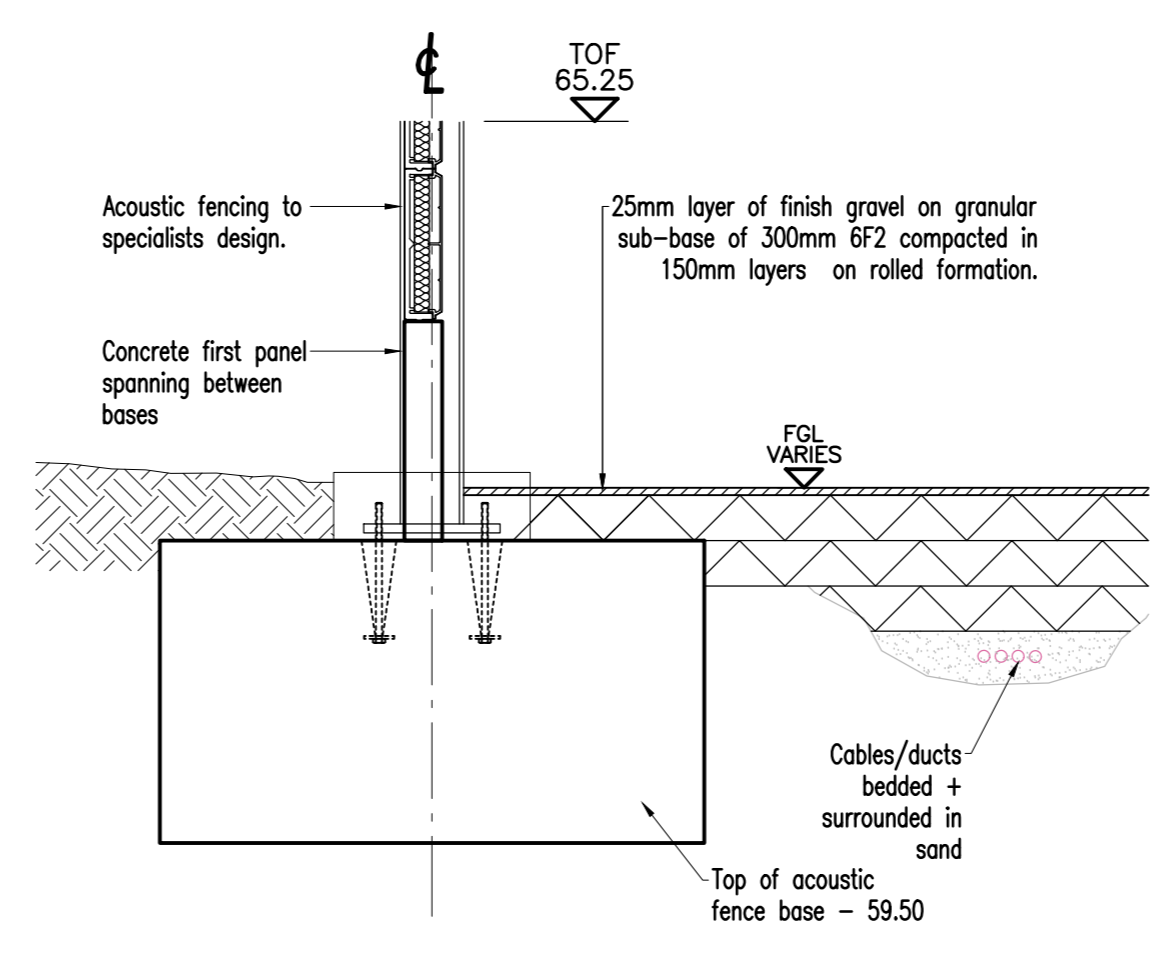
Typical Section Through Acoustic Fence
