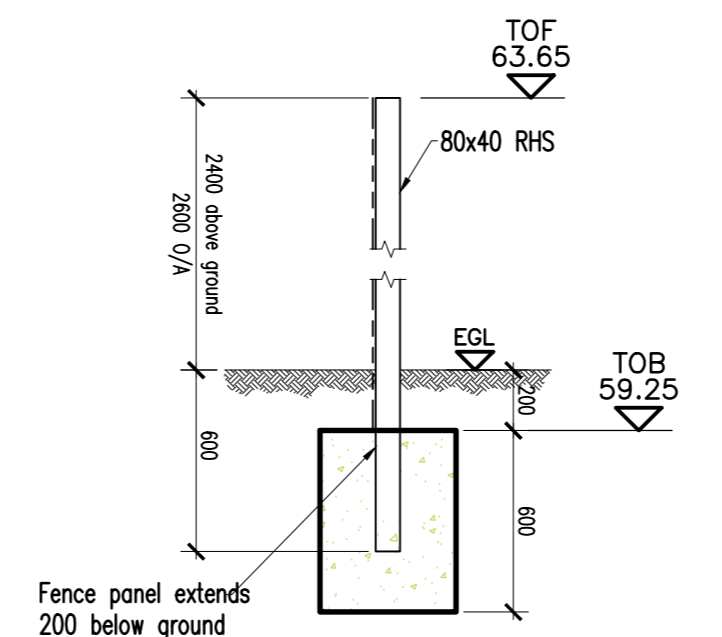
Typical Section Through Security Fence Base
