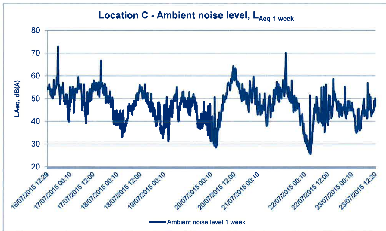
Graph 4: Location C - Long term unattended ambient noise level
