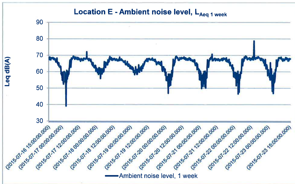
Graph 6: Location E - Long term unattended ambient noise level
