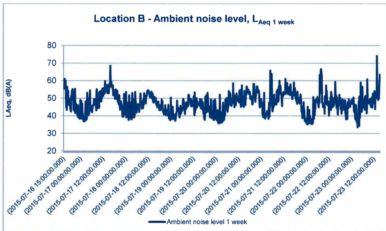
Graph 3: Location B - Long term unattended ambient noise level
