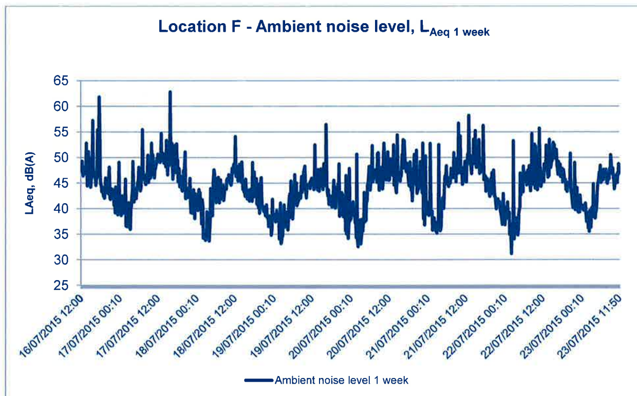
Graph 7: Location F - Long term unattended ambient noise level
