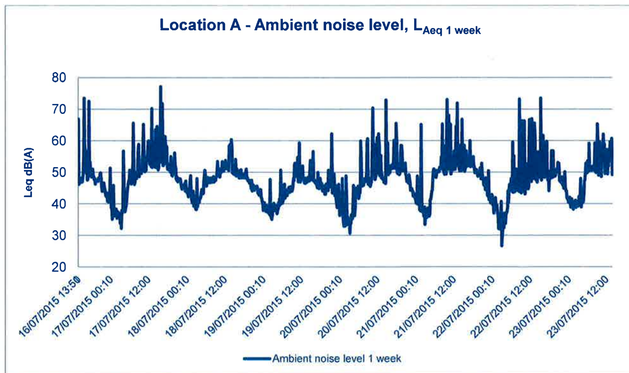
Graph 2: Location A - Long term unattended ambient noise level
