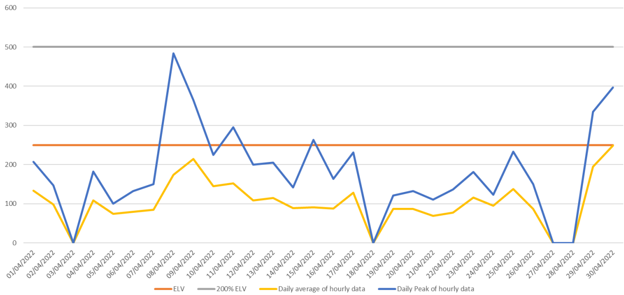
Summary of CO Emissions - Apr 2022
