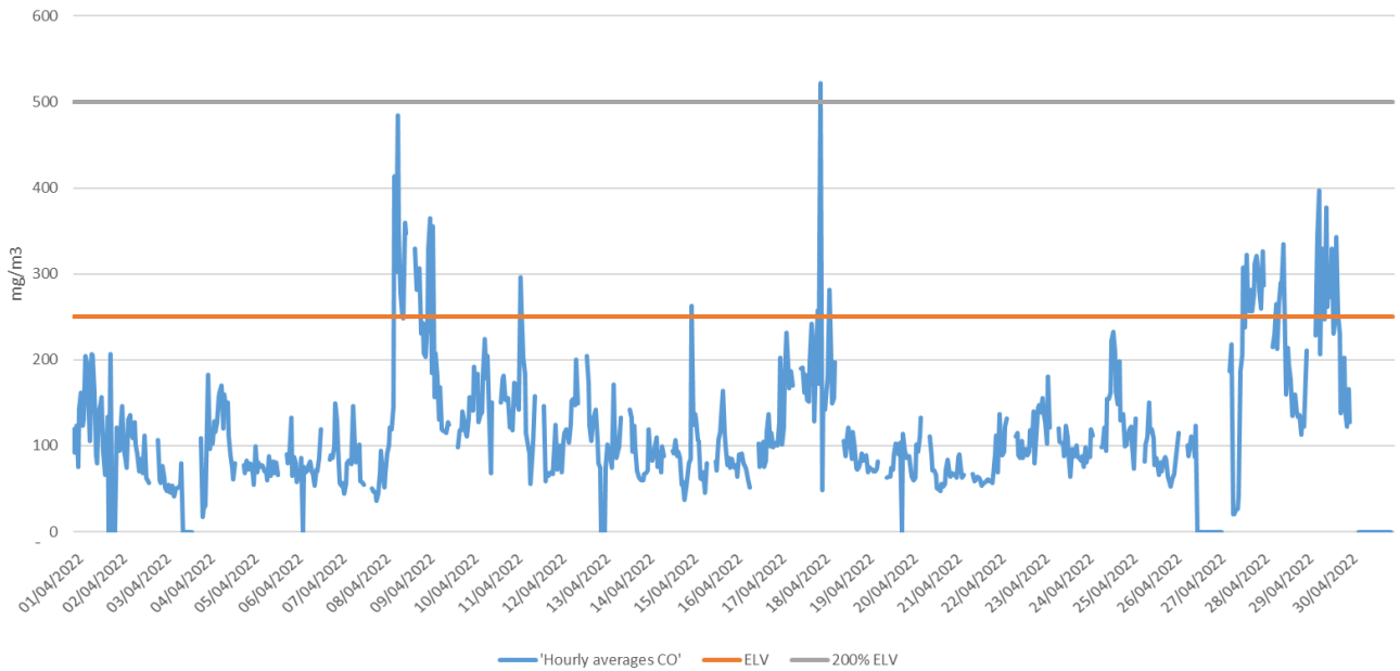
Summary of CO emission - Apr 2022
