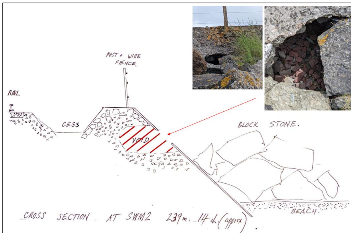
Figure 7: Breach to upper section of Ferryside North embankment.
