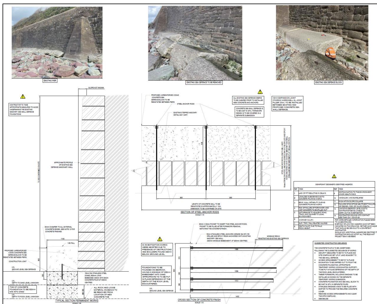
Figure 6: Toe repair design.
