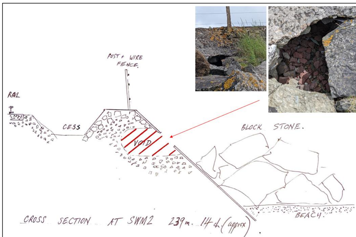
Figure 5: Breach to upper section of Ferryside North embankment.
