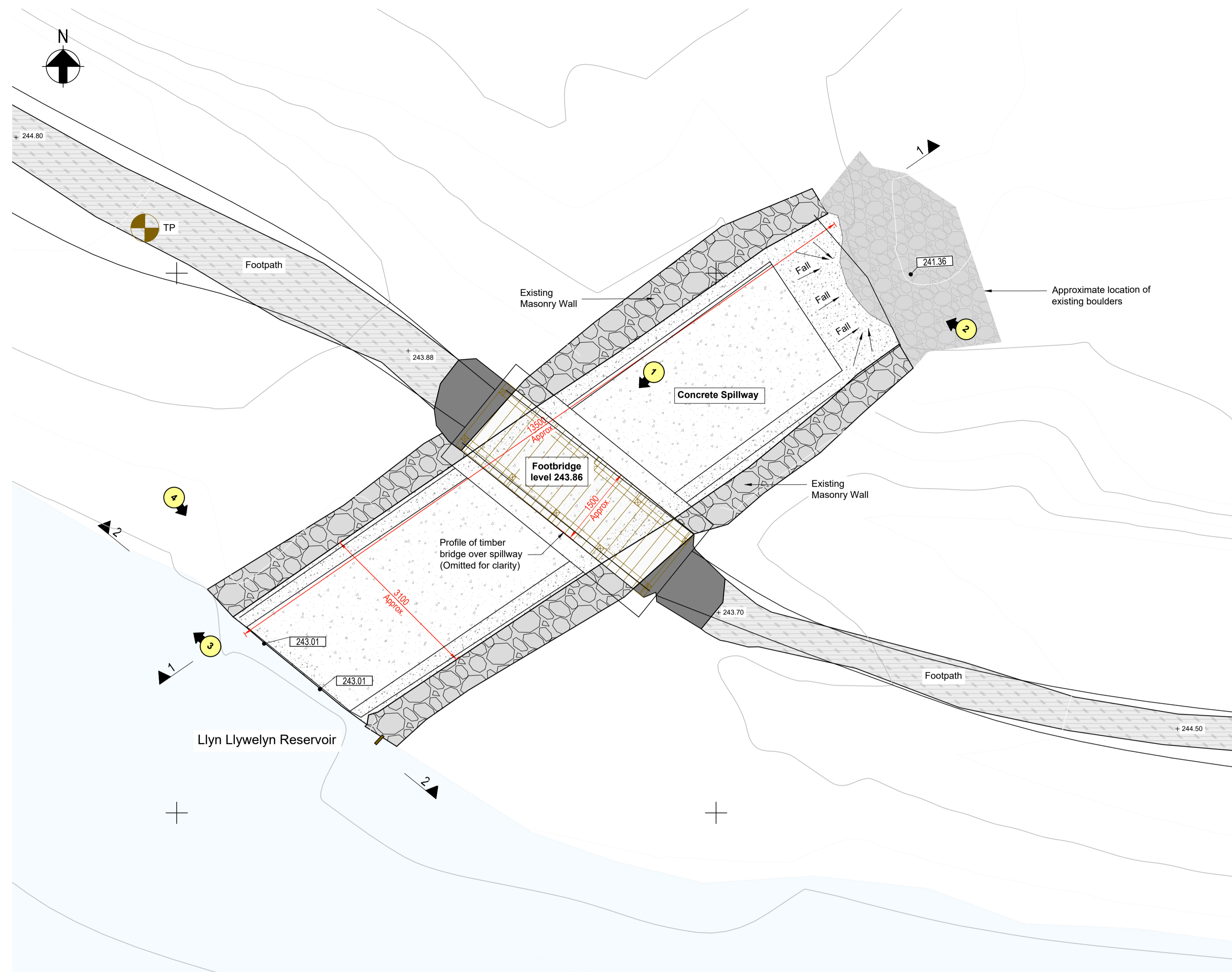
Plan of existing layout
