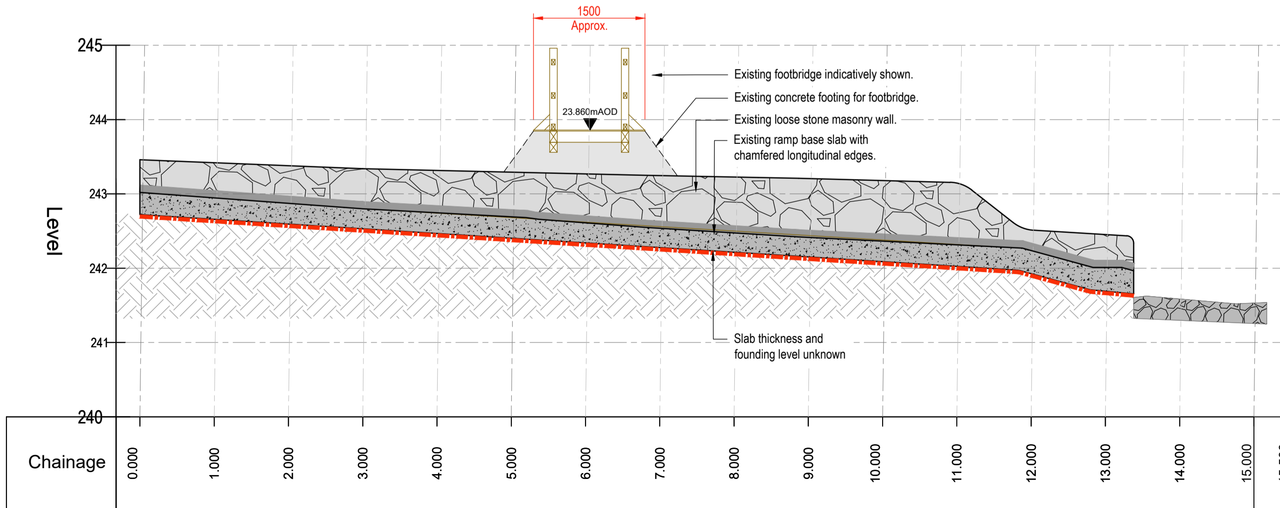
Section 1-1
