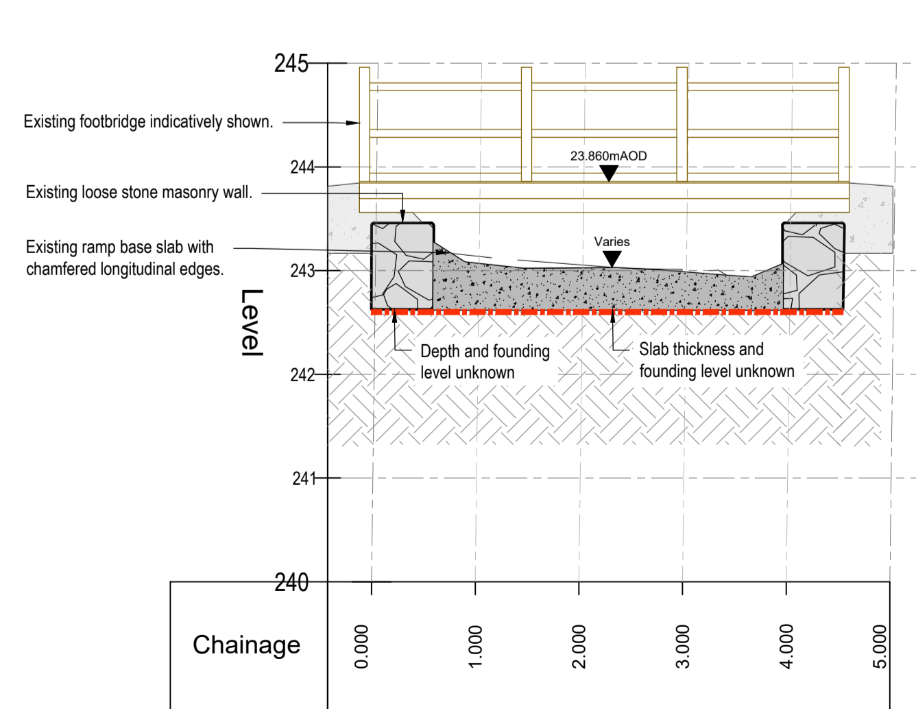
Section 2-2
