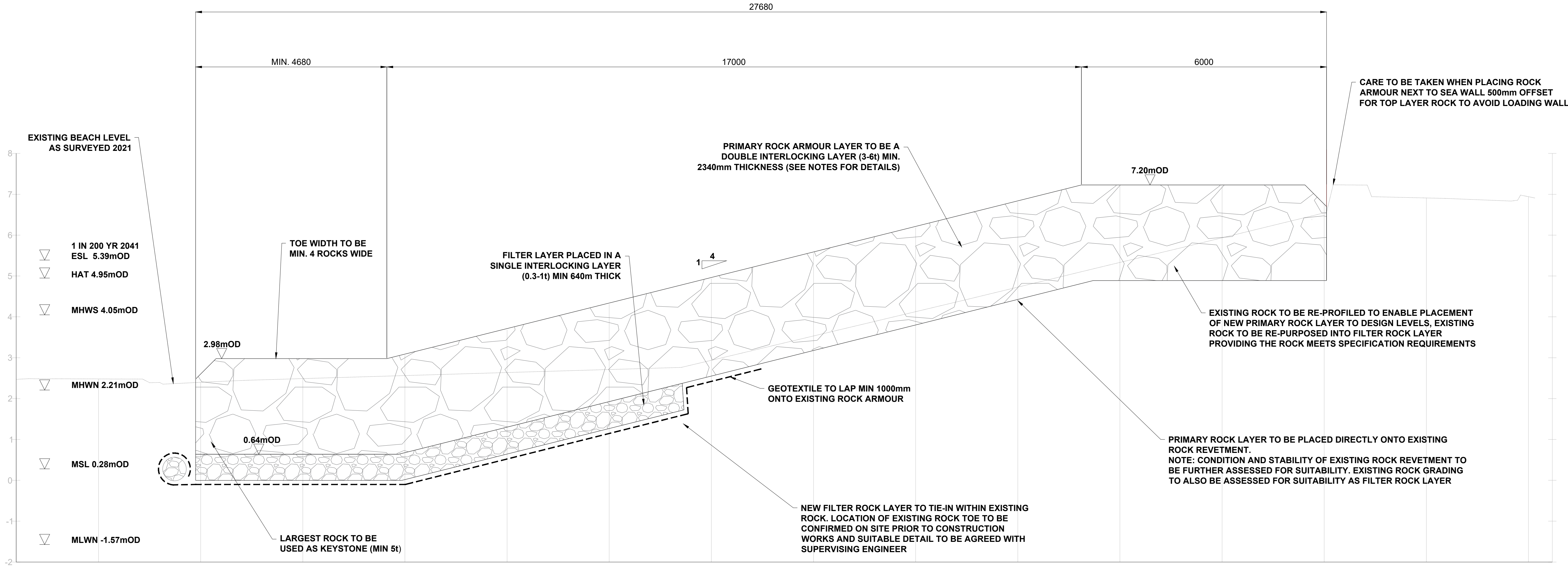
TYPICAL SECTION TYPE A
