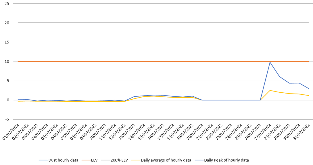
Summary of Particulate Emissions - Jul 2022
