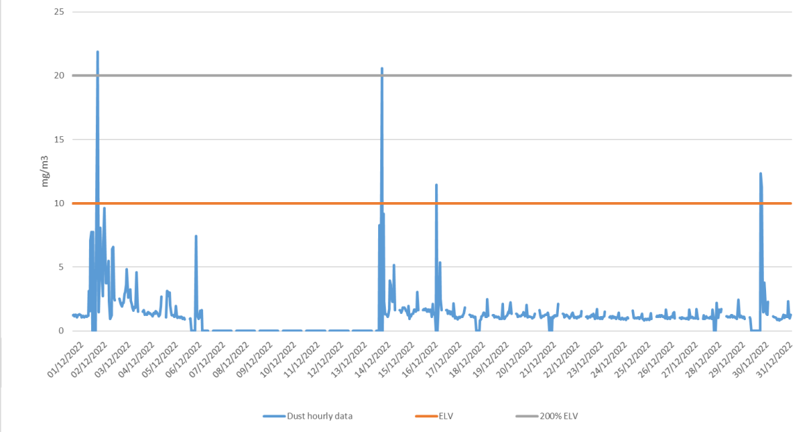
Summary of Particulate Emission - Dec 2022
