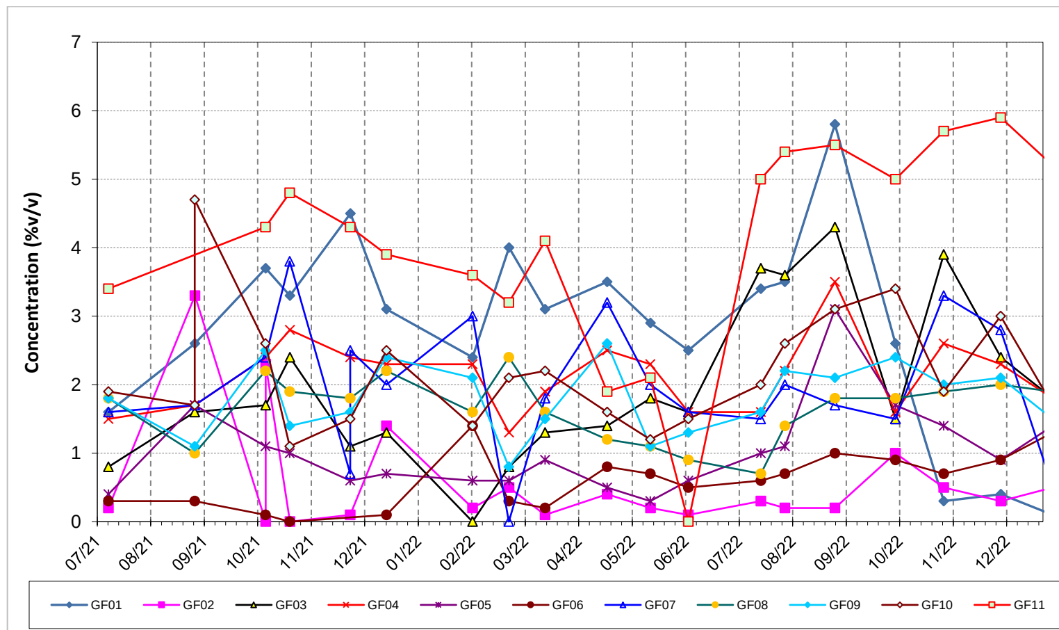
Figure 3.2 In waste carbon dioxide concentrations in since boreholes were drilled (July 2021)
