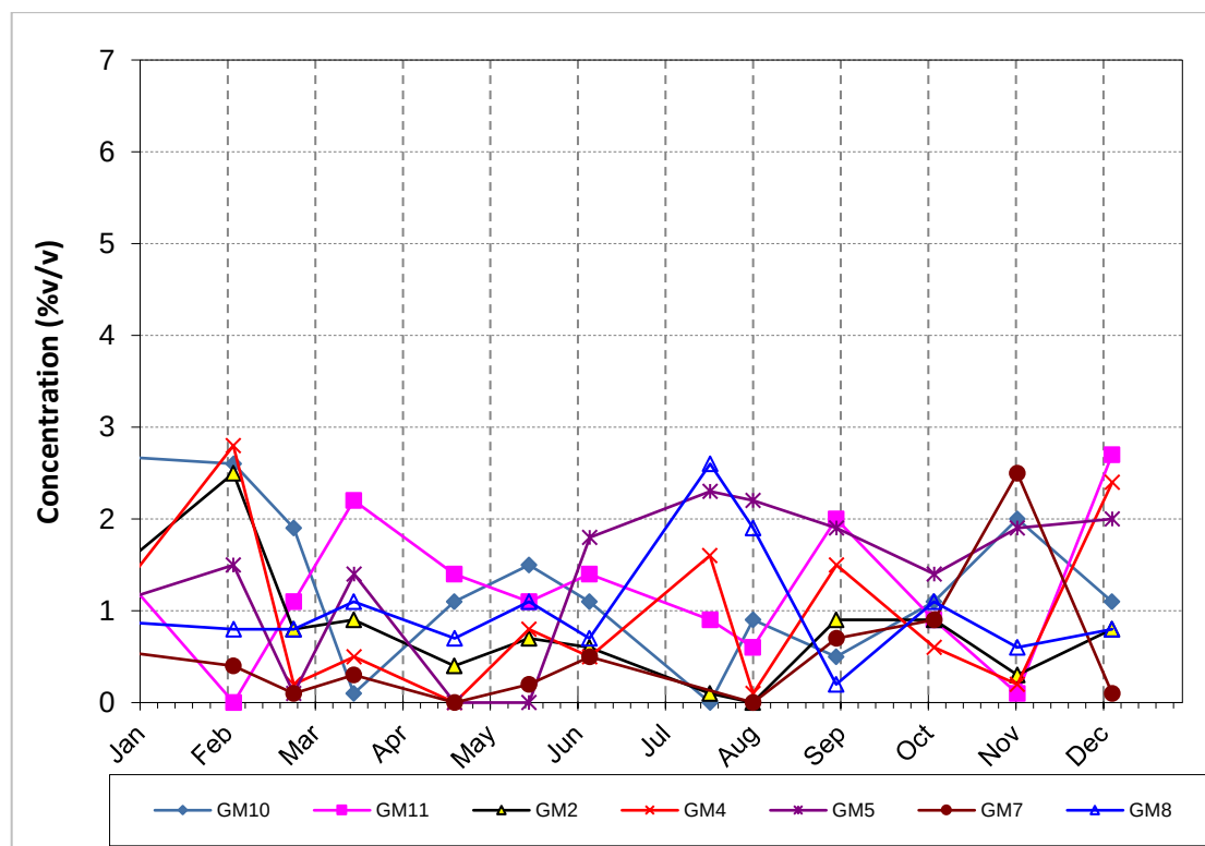
Figure 3.4 Stable carbon dioxide concentrations in 2022
