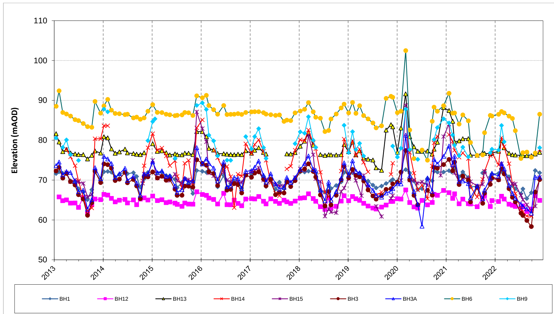
Figure 3.7 Historical groundwater elevation (2013-2022)
