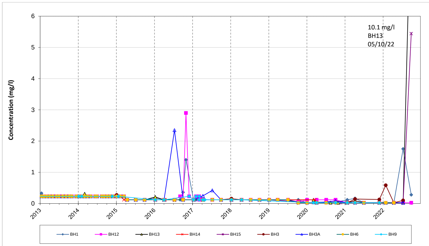
Figure 3.12 Historical iron concentrations at all groundwater locations
