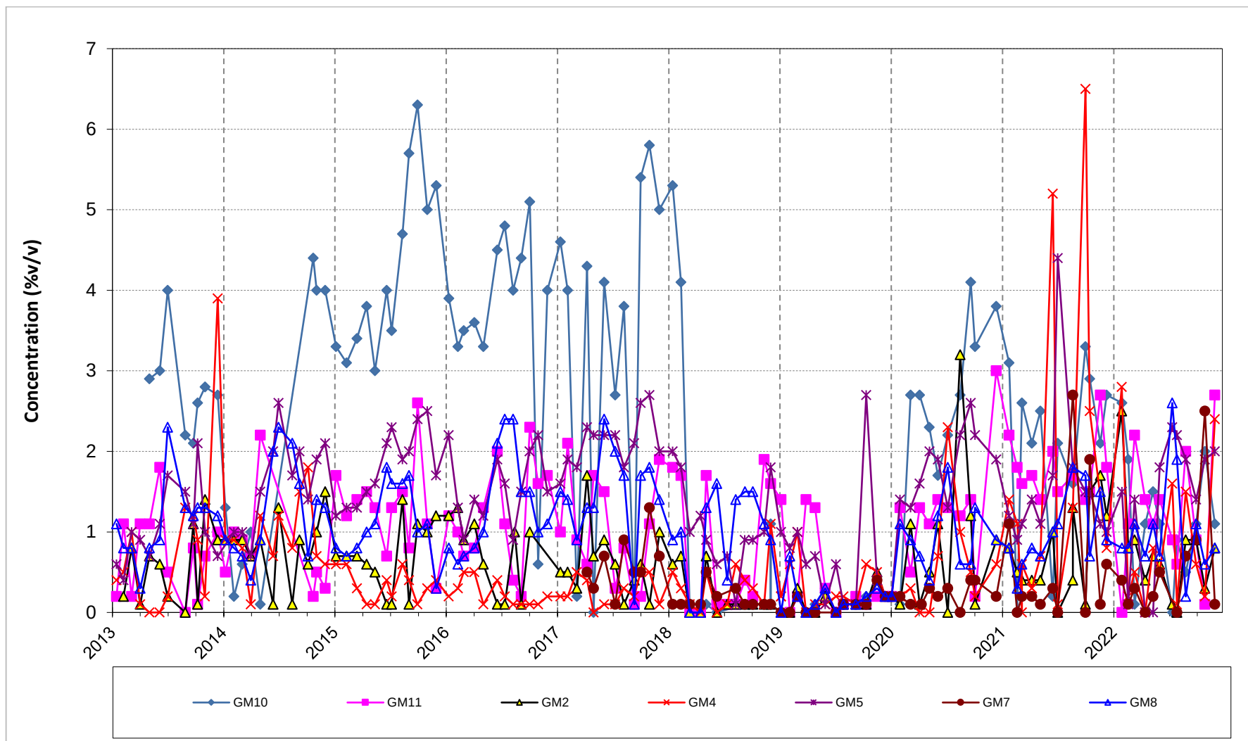
Figure 3.5 Historical stable carbon dioxide concentrations
