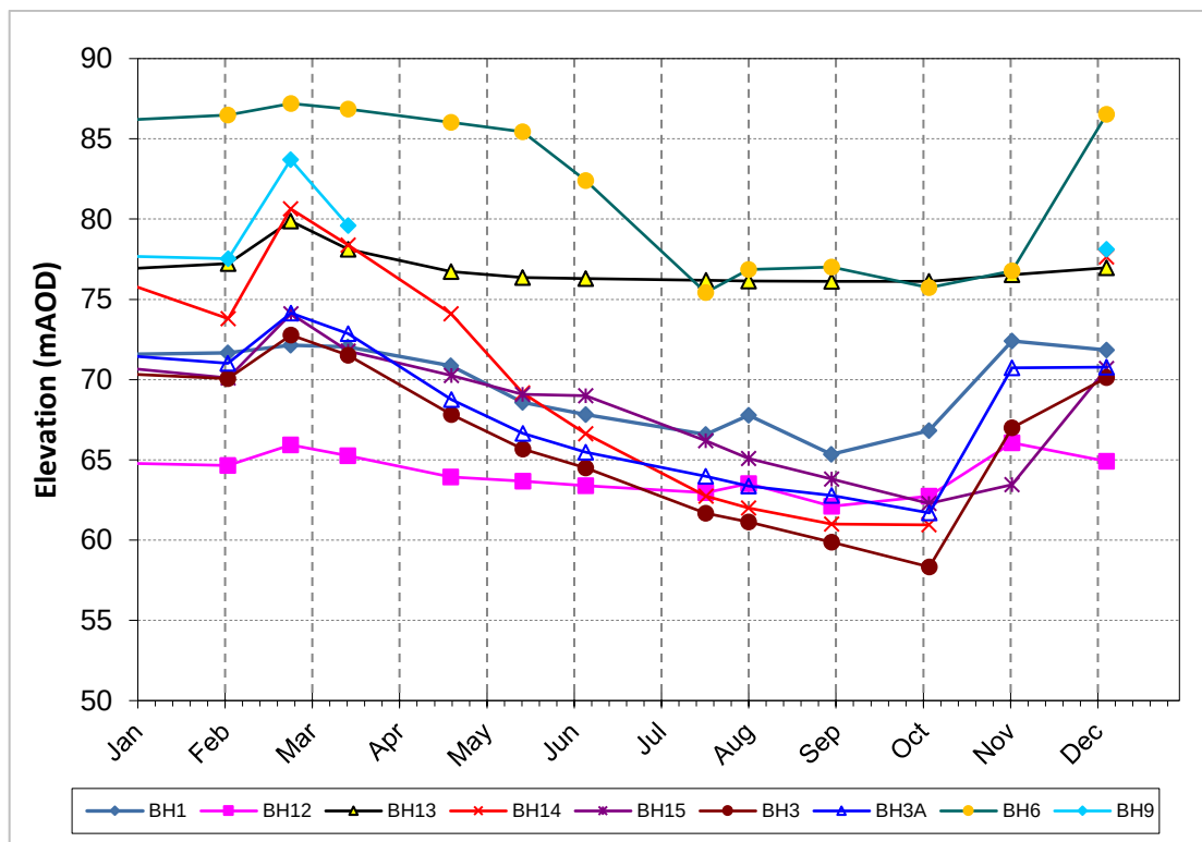
Figure 3.6 Groundwater elevation during 2022
