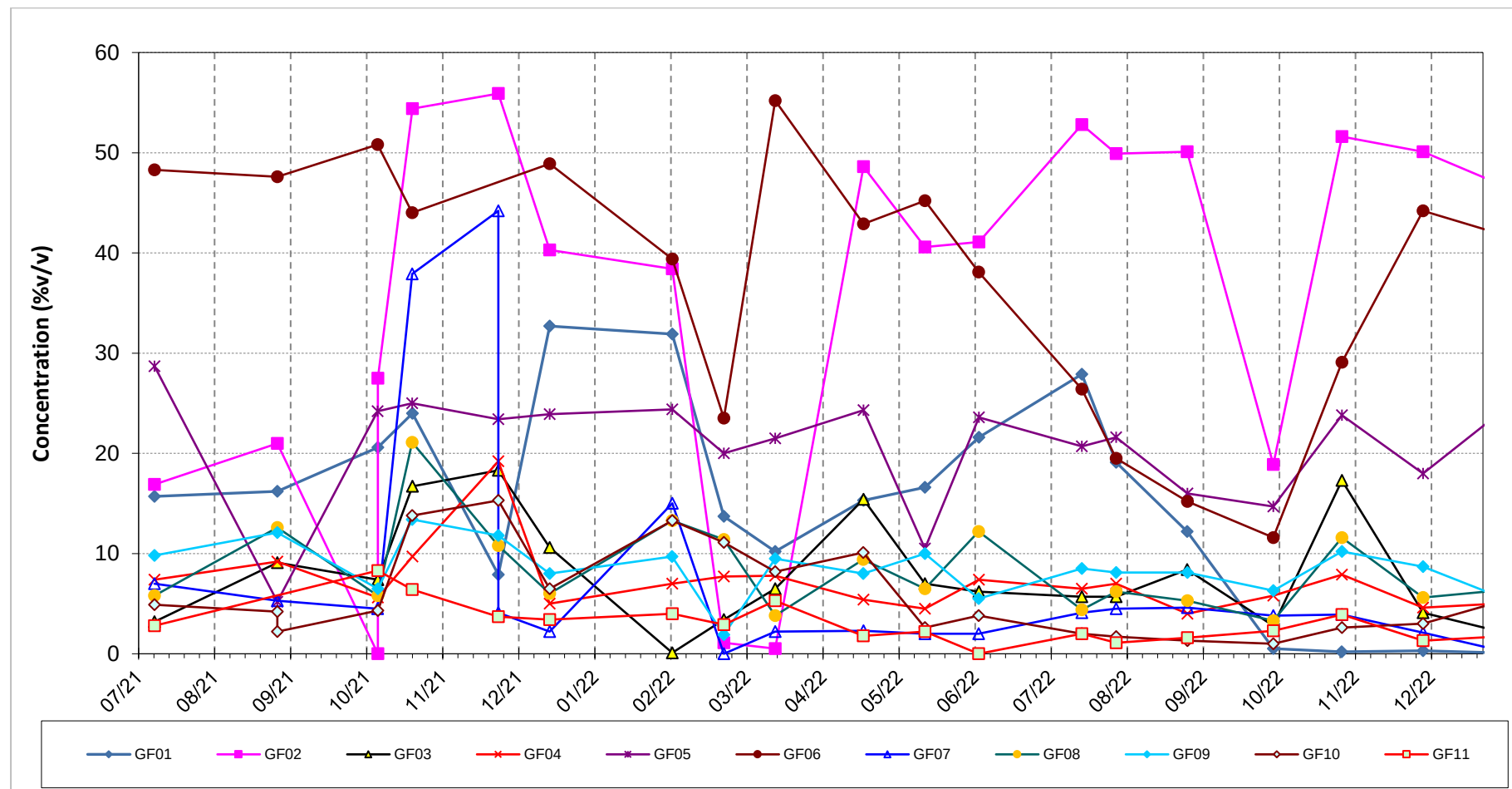
Figure 3.1 In-waste stable methane concentrations since boreholes were drilled (July 2021)
