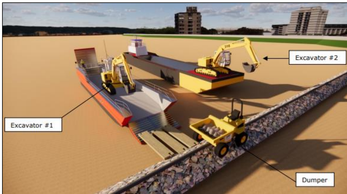
Figure 3 Illustration of working configuration during decommissioning of the existing pipe (reproduced from Kaymac 2022b).
