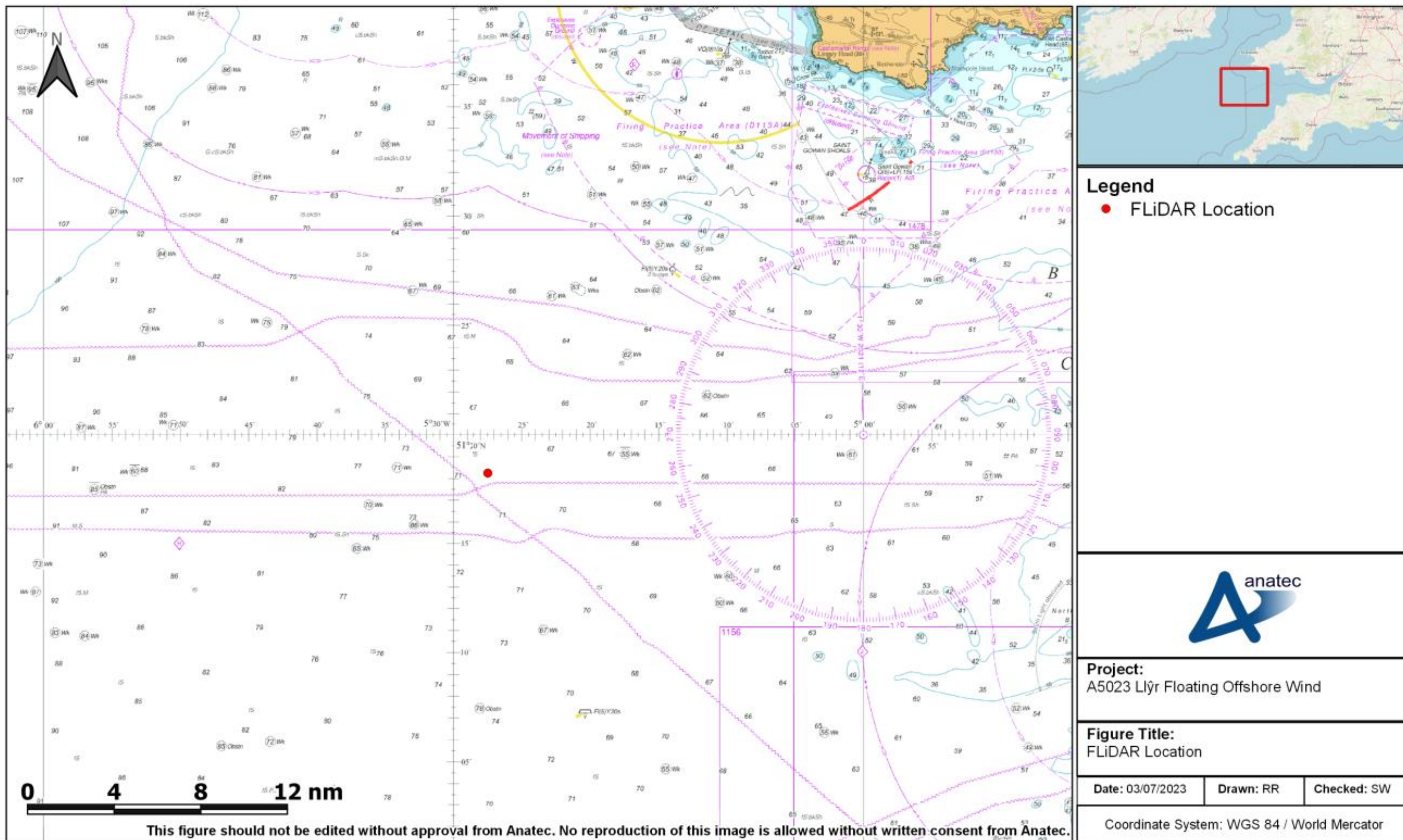
Figure 1. Location of floating LiDAR (FLiDAR)
