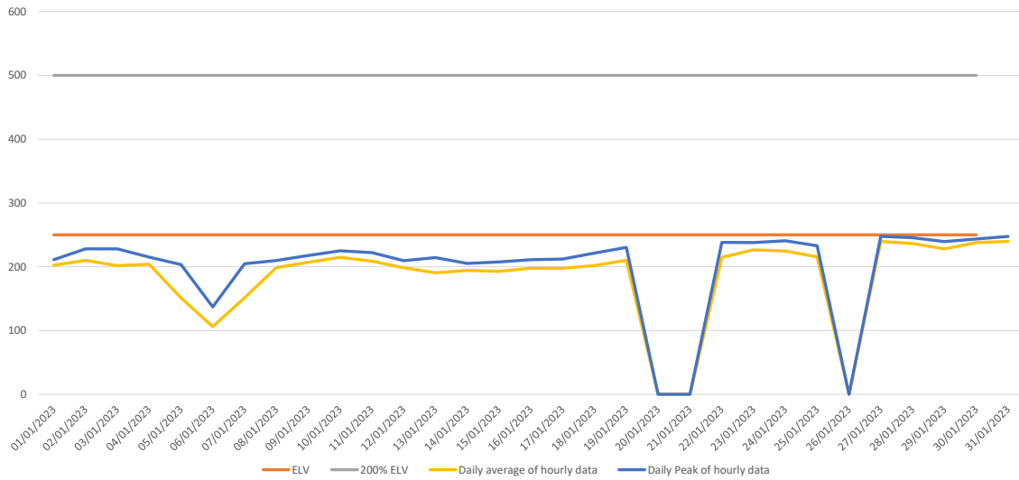
Summary of Nox Emissions - Jan 2023
