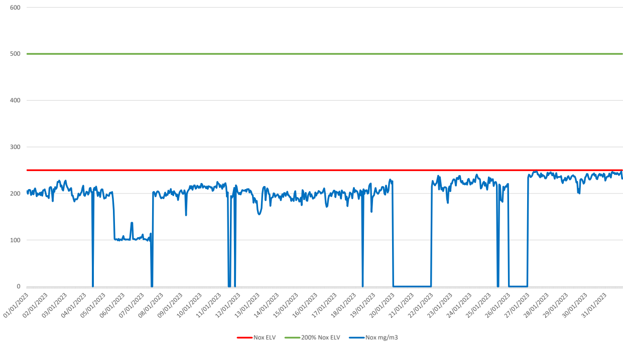
Summary of Nox Emissions - Jan 2023
