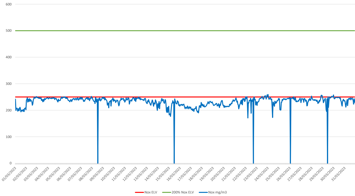
Summary of Nox Emissions - Mar 2023
