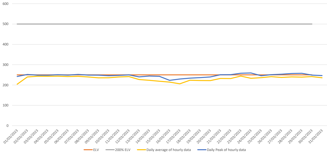
Summary of Nox Emissions - Mar 2023
