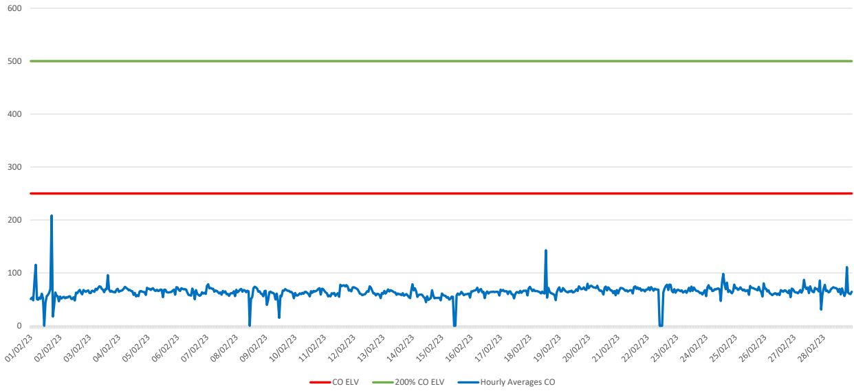
Summary of CO Emissions - Feb 2023
