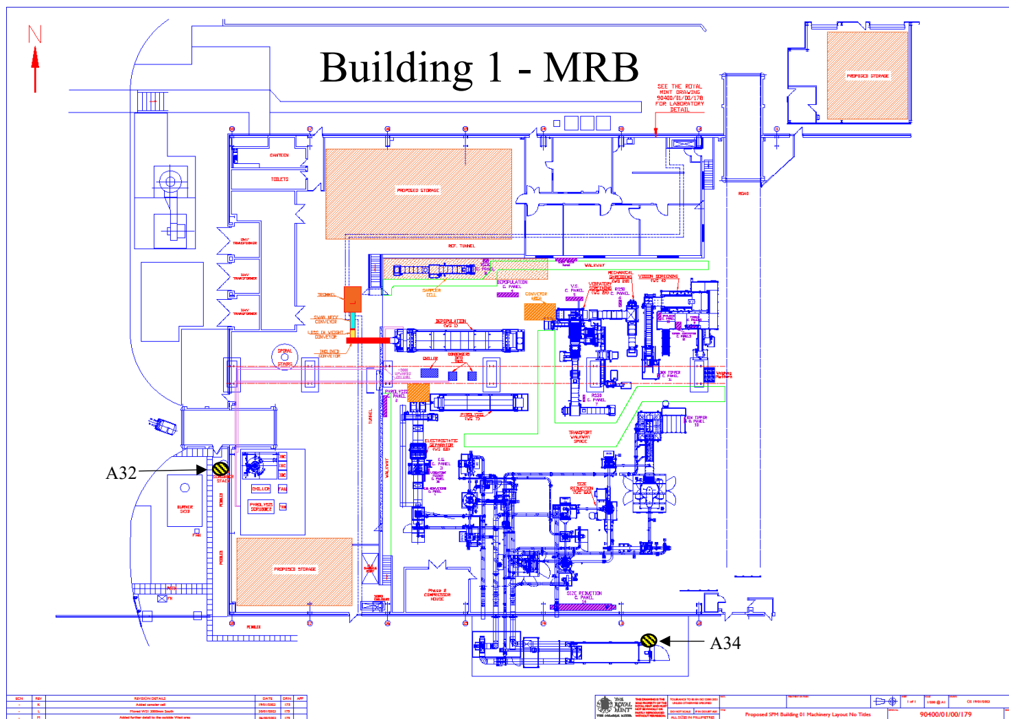
Figure 1.3: Site Layout – MRB Building
