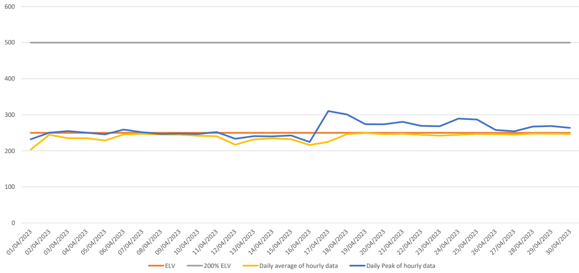
Summary of Nox Emissions - Apr 2023
