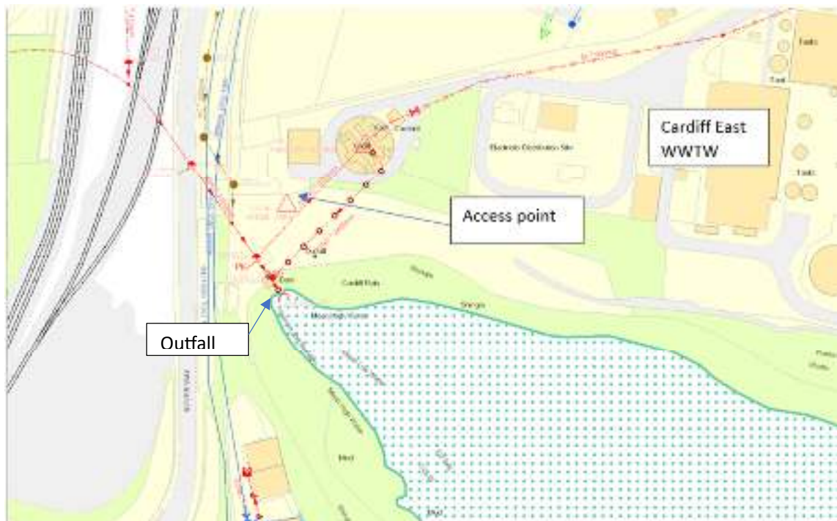
Figure 1 – GIS plan of location.
