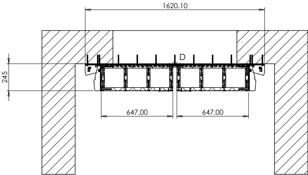
SECTION B-B
