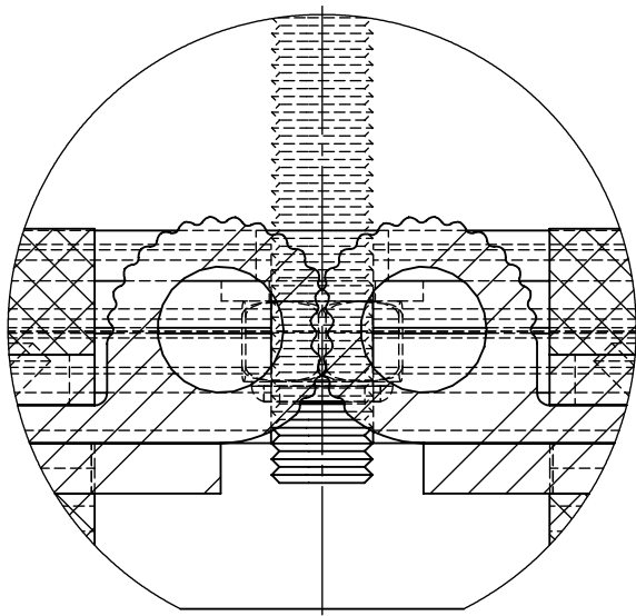
Centre seal Detail D SCALE 3 : 2
