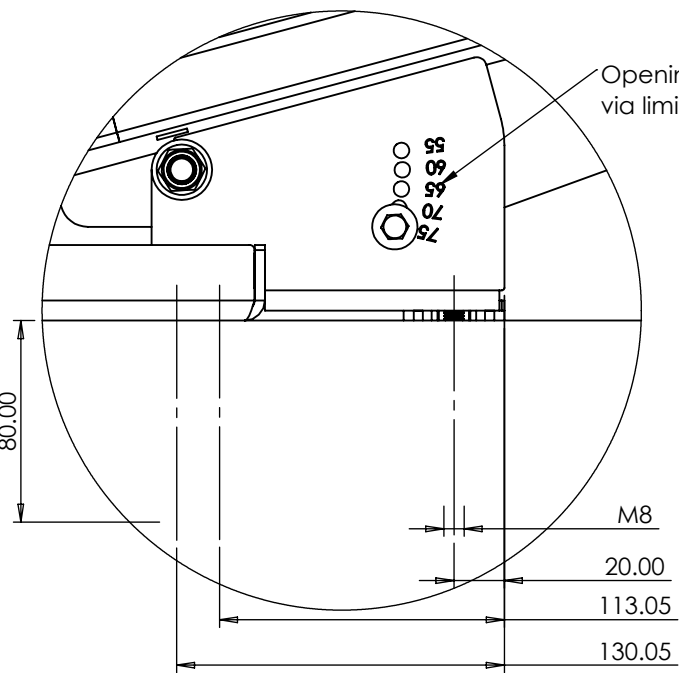
Hinge Detail E SCALE 1 : 3
