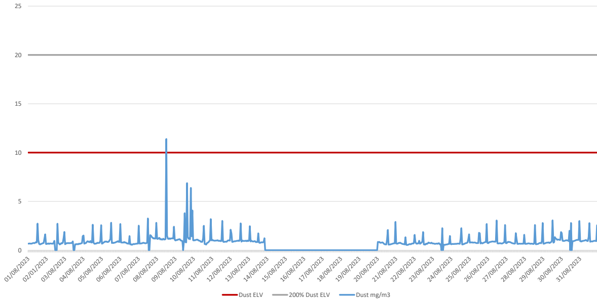
Summary of Particulate Emissions - Aug 2023
