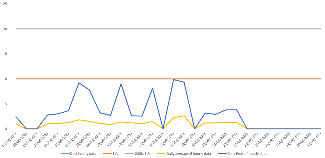
Summary of Particulate Emissions - Sep 2023
