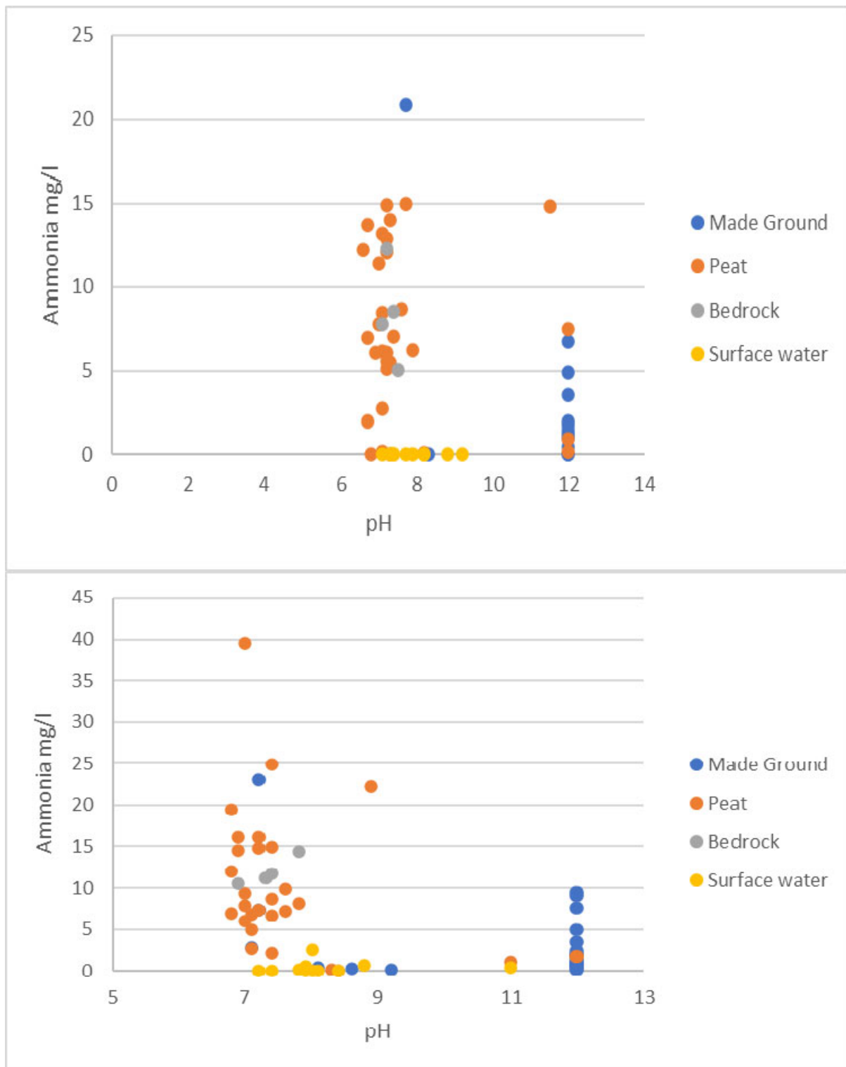
Plate 5-2 Ammonia concentrations during 2020 (top) and 2021 (bottom)
