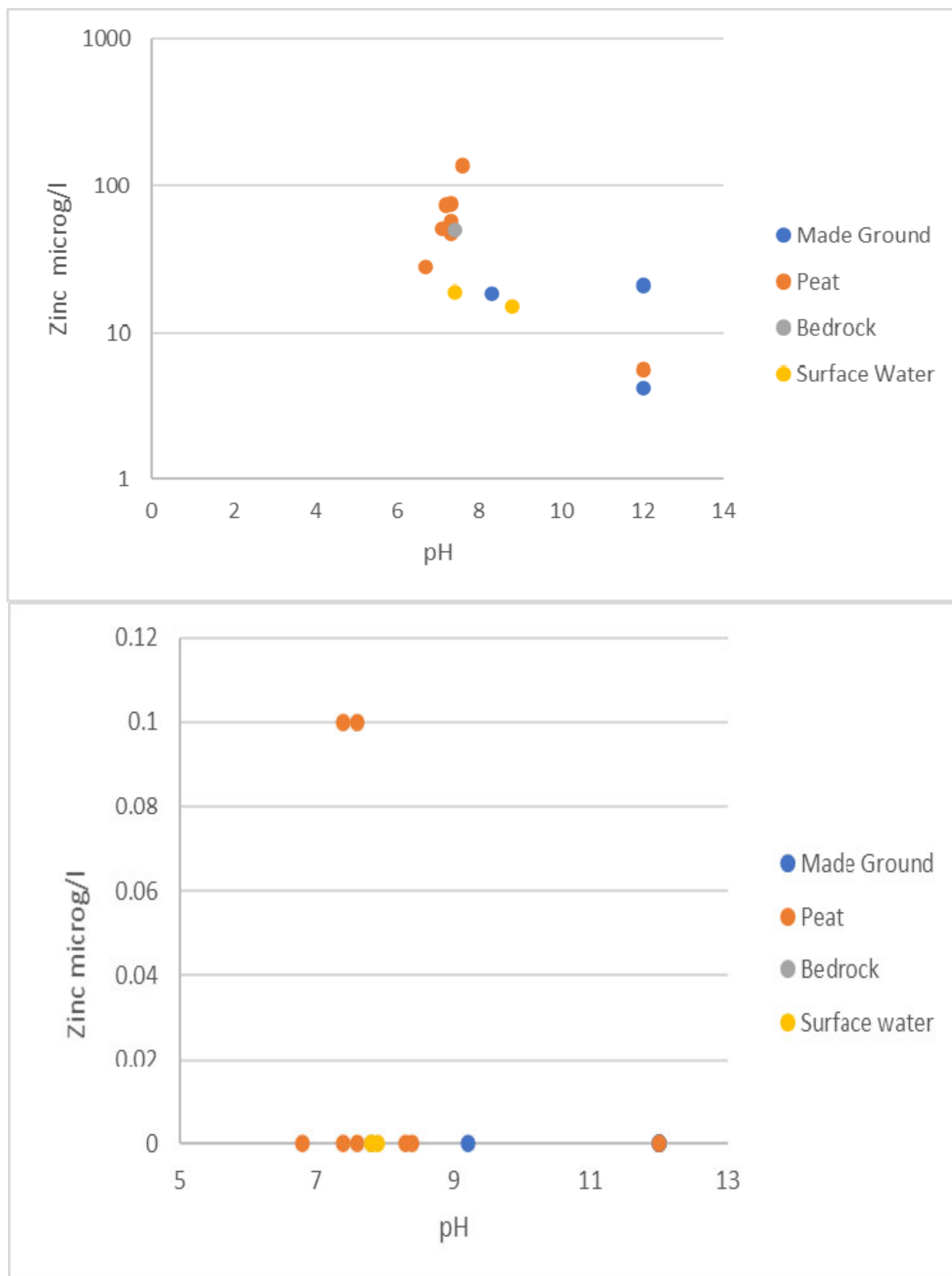
Plate 5-4 Zinc concentration during 2020 (top) and 2021 (bottom)
