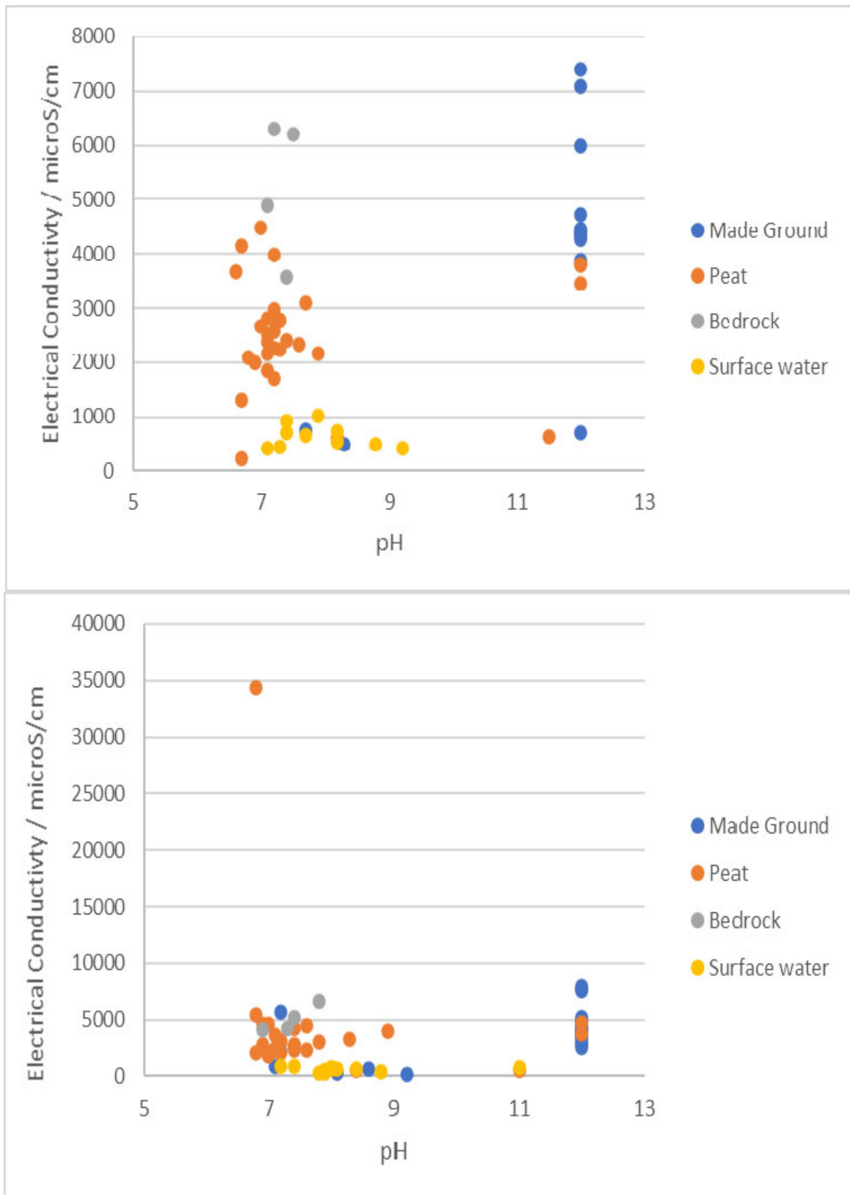
Plate 5-1 pH and Electrical Conductivity during 2020 (top) and 2021 (bottom)
