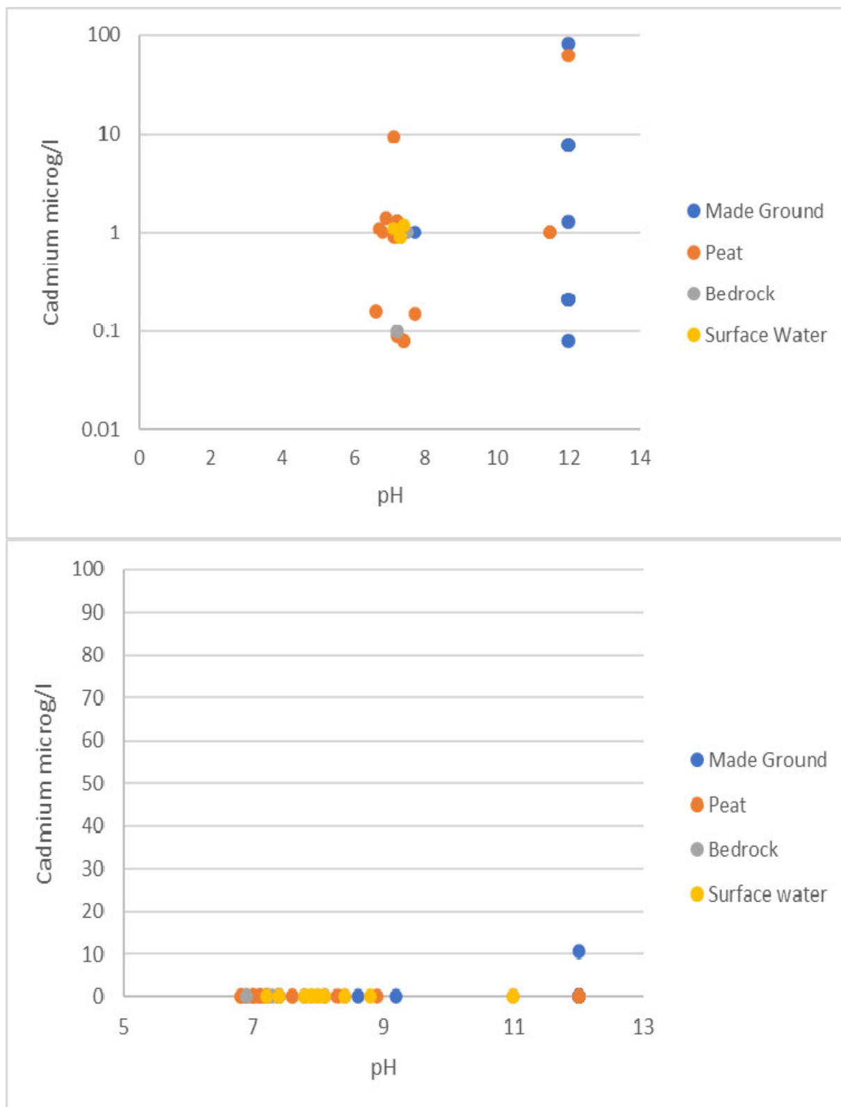
Plate 5-3 Cadmium concentration during 2020 (top) and 2021 (base)
