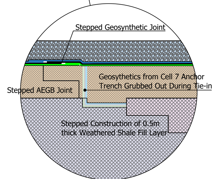
Inset Showing Stepped Joint Construction Detail
