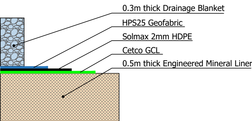
Lining Build-up
