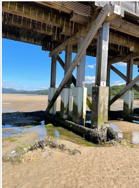
Areas of new timbers and repairs
