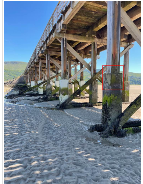
Repairs at span 30
