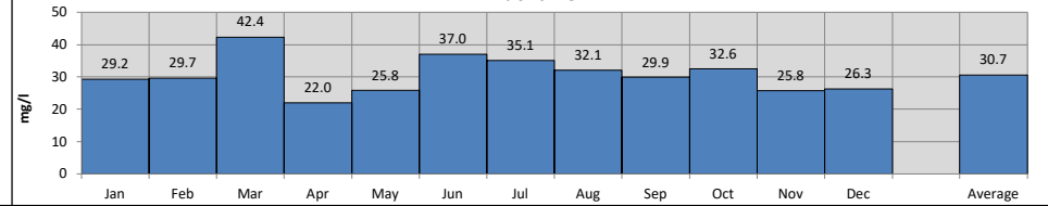
Effluent suspended solids
