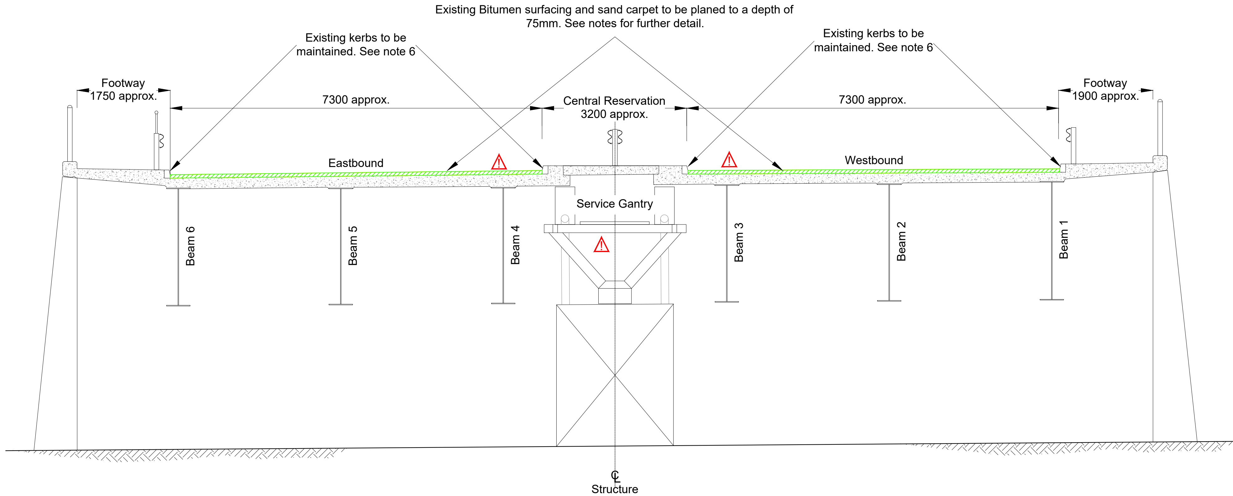
CROSS SECTION (Indicative only) Scale 1:50
