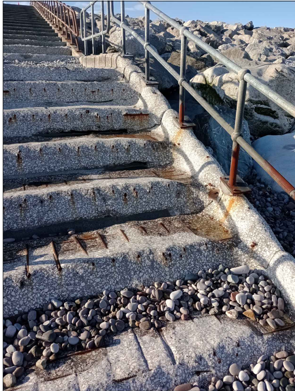
PHOTO 3 - VIEW OF EXPOSED REBAR ON RIGHT OF STAIRCASE
