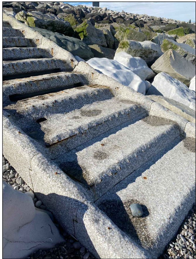
PHOTO 3 - VIEW OF BOTTOM STAIRCASE WITH EXPOSED REBAR
