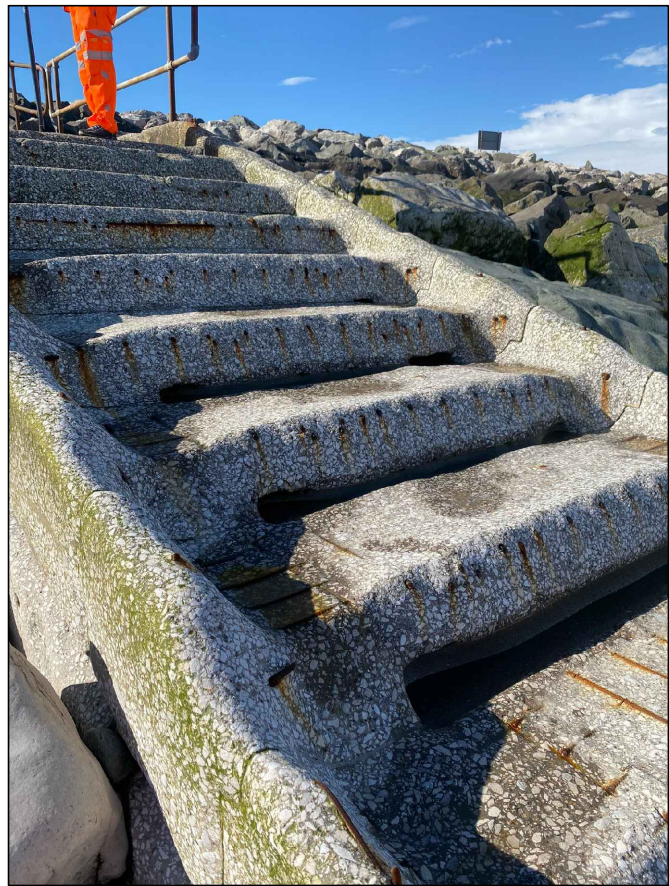
PHOTO 2 - VIEW OF HALFWAY OF BOTTOM STAIRCASE WITH EXPOSED REBAR
