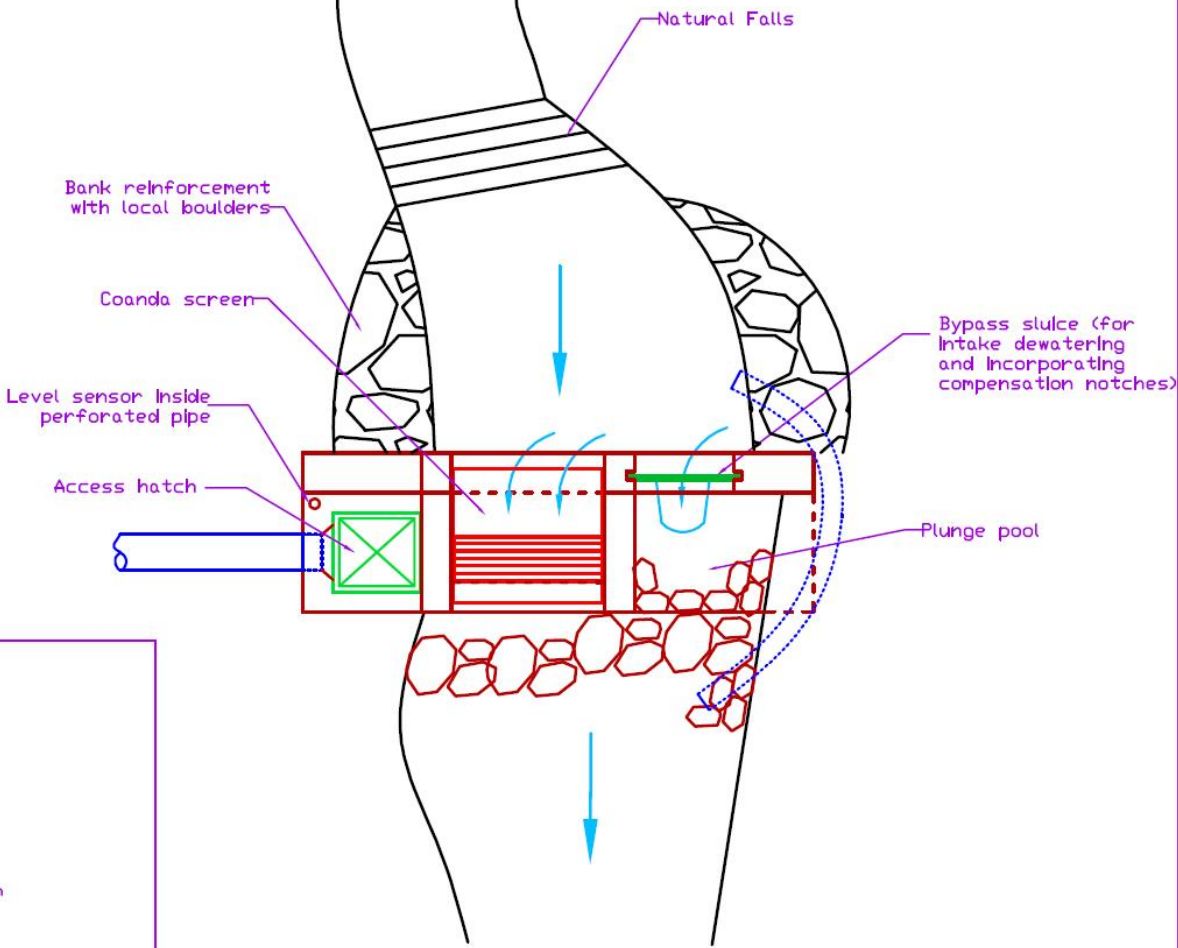
SIDE ELEVATION (A-A) Coanda
