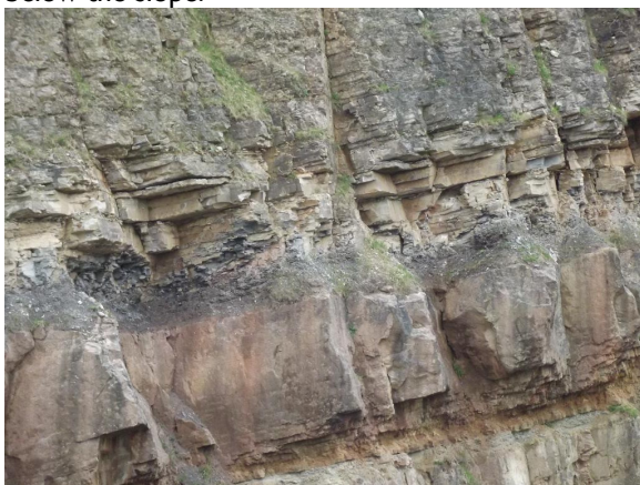
Plate 12: Close-up of preferential weathering along soft shaley bands
