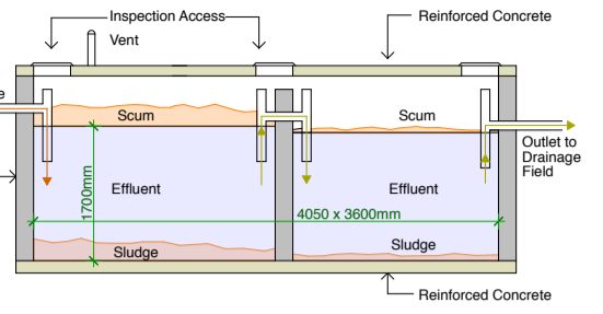
Typical Septic Tank Detail Dimension are approximate Septic Tank 1 - generally as above Septic Tank 2 - generally as above x 2
