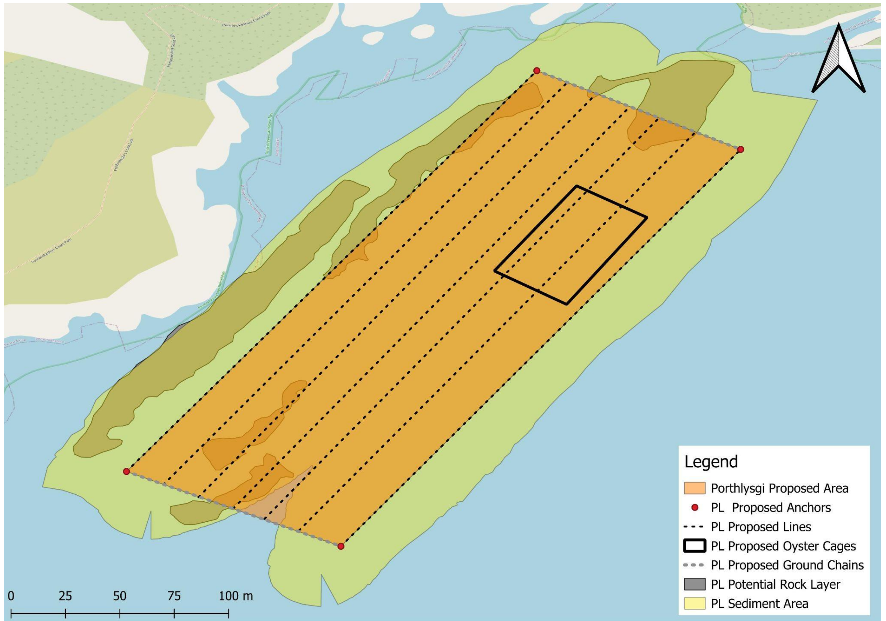
Figure 17 - Porthlysgei Proposed Farm Sonar Habitat Map
