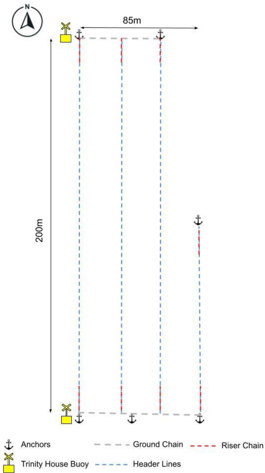
Carn Ar Wig Farm Design
