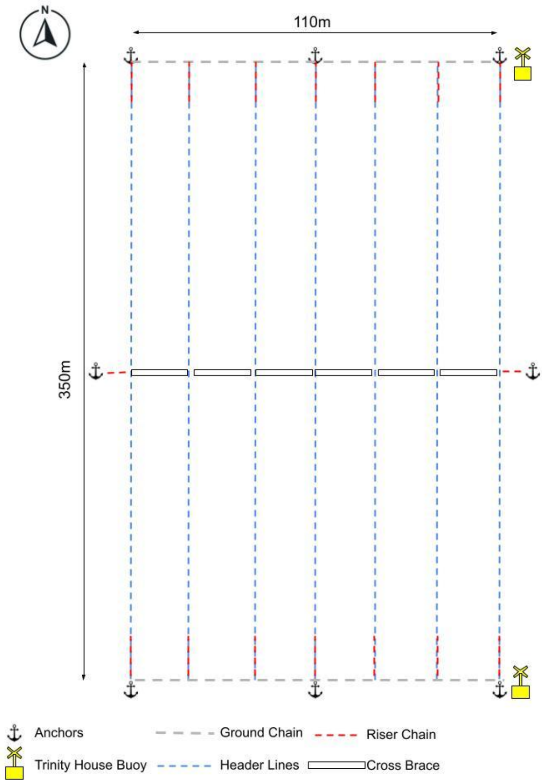
Porthlysgi Farm Design
