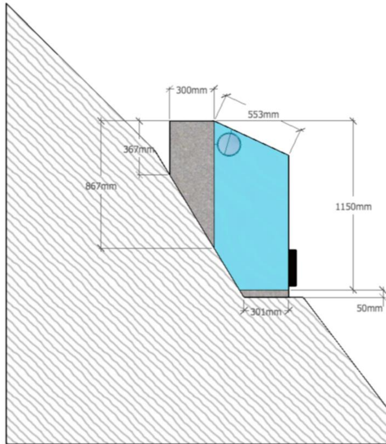
Proposed Micro Hydro Scheme, Llyndy Isaf Intake 1 TCV Hydro Ltd CRIC, Beaufort Street Crickhowell Powys, NP8 1BN TCV 13-010-07 Intake 1 cross section A4 1:20
