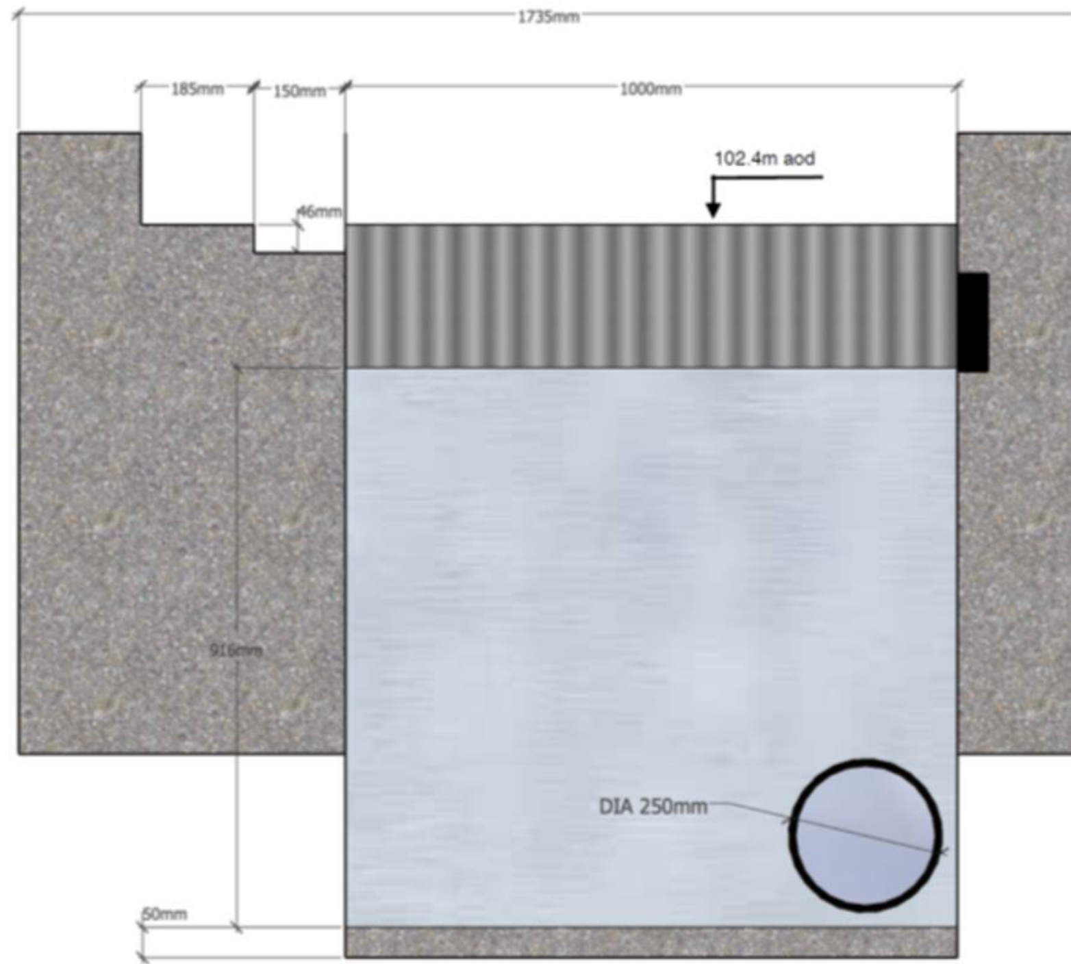
Proposed Micro Hydro Scheme, Llyndy Isaf Intake 1 ( revised HOF notch) TGV Hydro Ltd CRIC, Beaufort Street Crickhowell Powys, NP8 1BN TGV 13-010-06 Revision 1 Intake 1 front elevation A4 1:20
