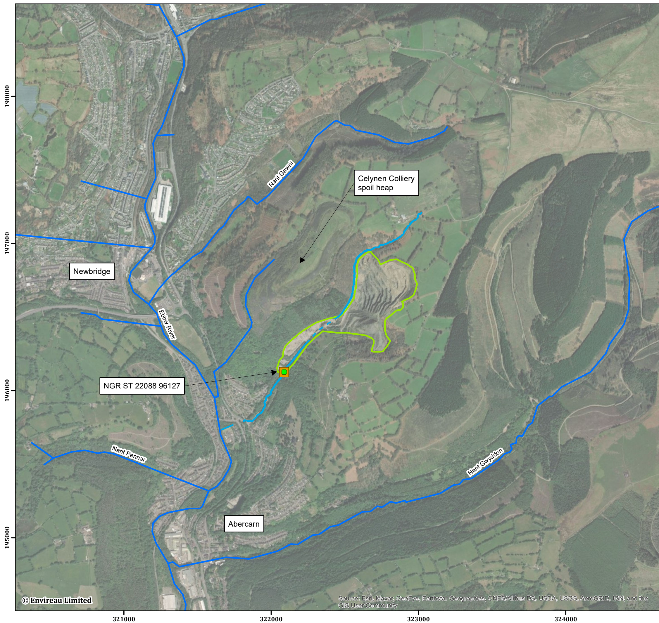
Figure 1: Site Setting
