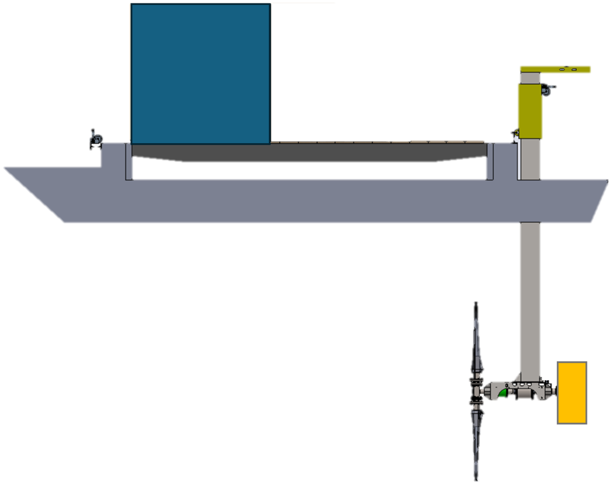
Figure 2 Device in operational position (Not to scale)
