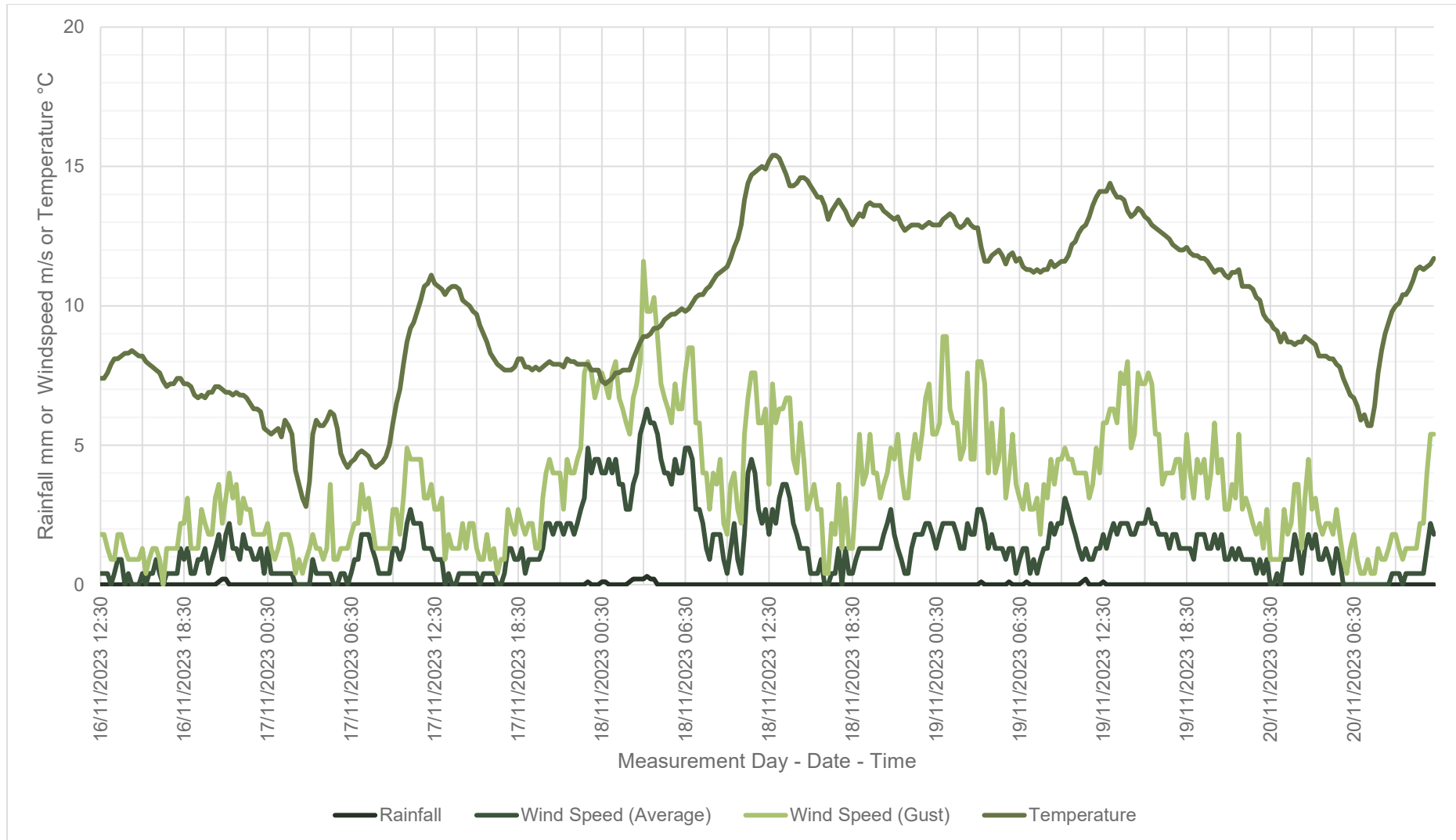
Figure C-1: Weather Overview
