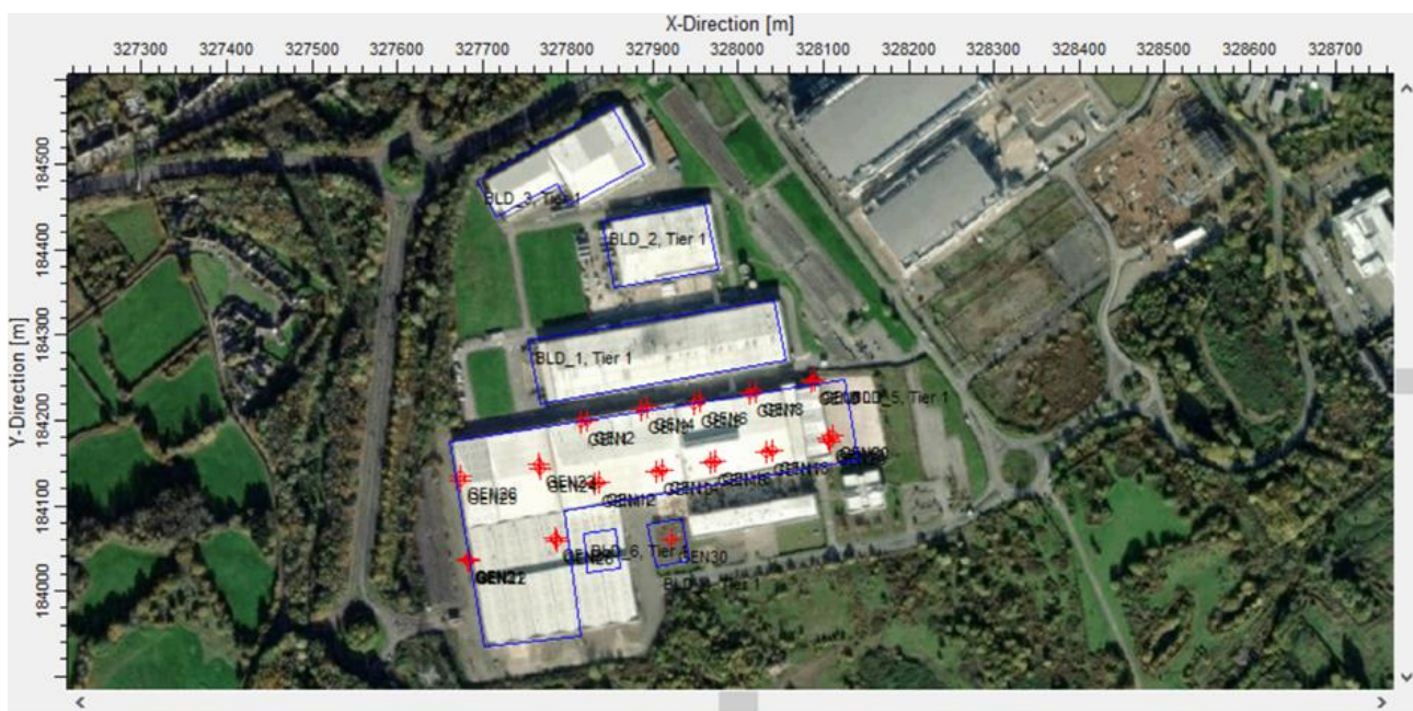
FIGURE 6-1 SITE LAYOUT – EMISSION SOURCES
