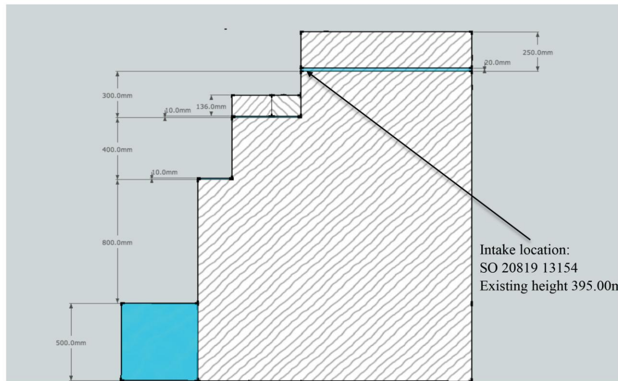
Intake - Existing Profile View
