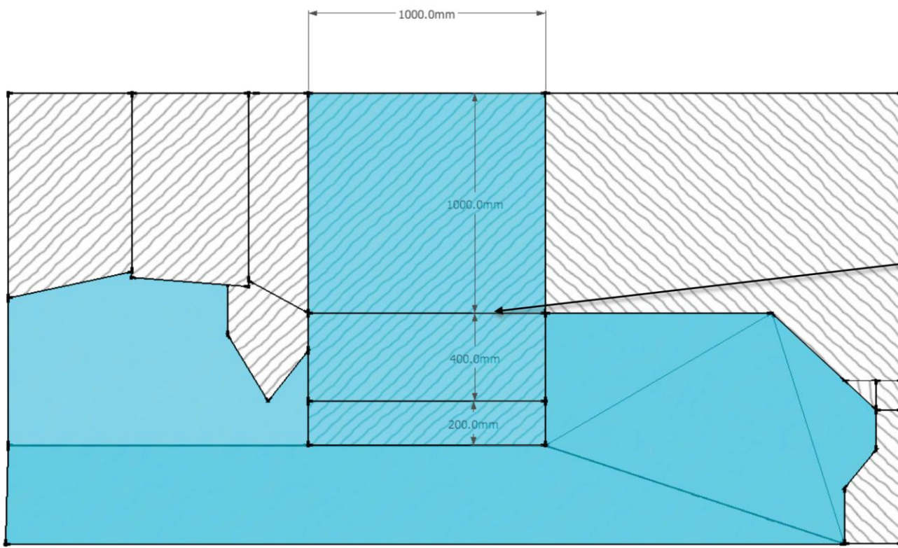
Intake - Existing Plan View
