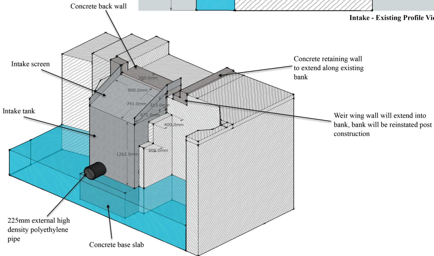
Intake - Proposed Isometric View
