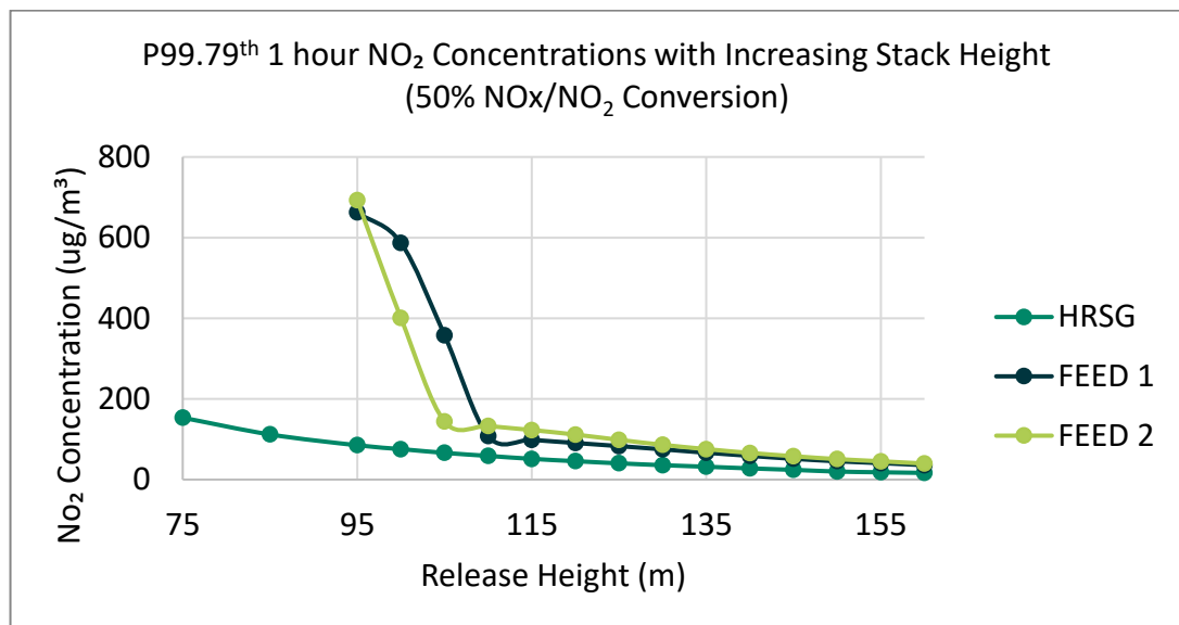
Plate 2: Predicted Maximum Process Contribution to Ground Level NO 2 Concentrations at Stack Release Heights of 75 m to 160 m
