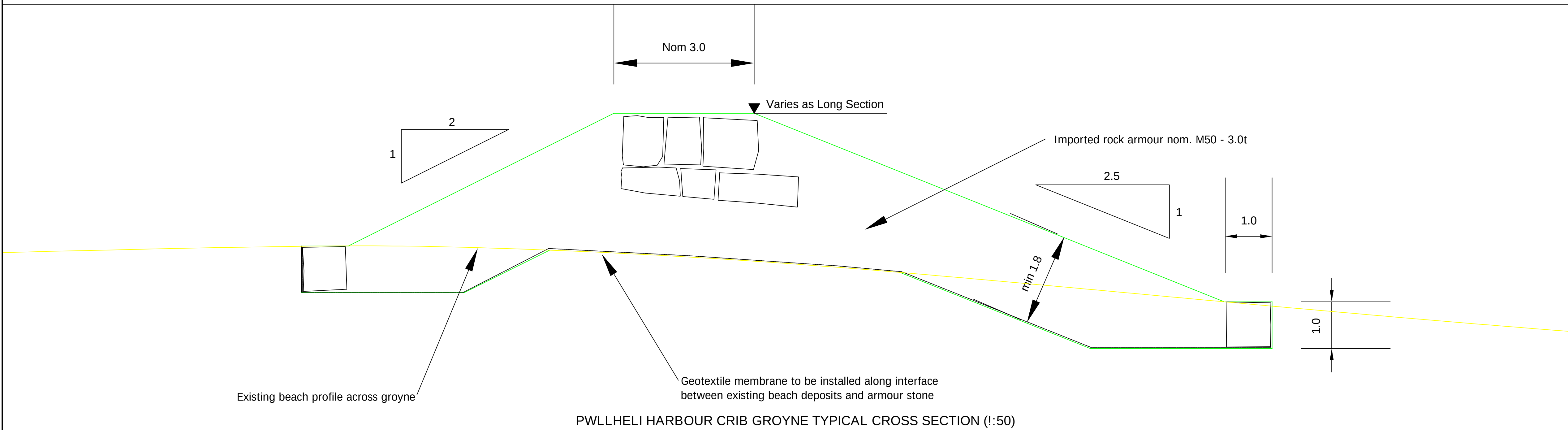
PWLLHELI HARBOUR CRIB GROYPE TYPICAL CROSS SECTION (1:50)
