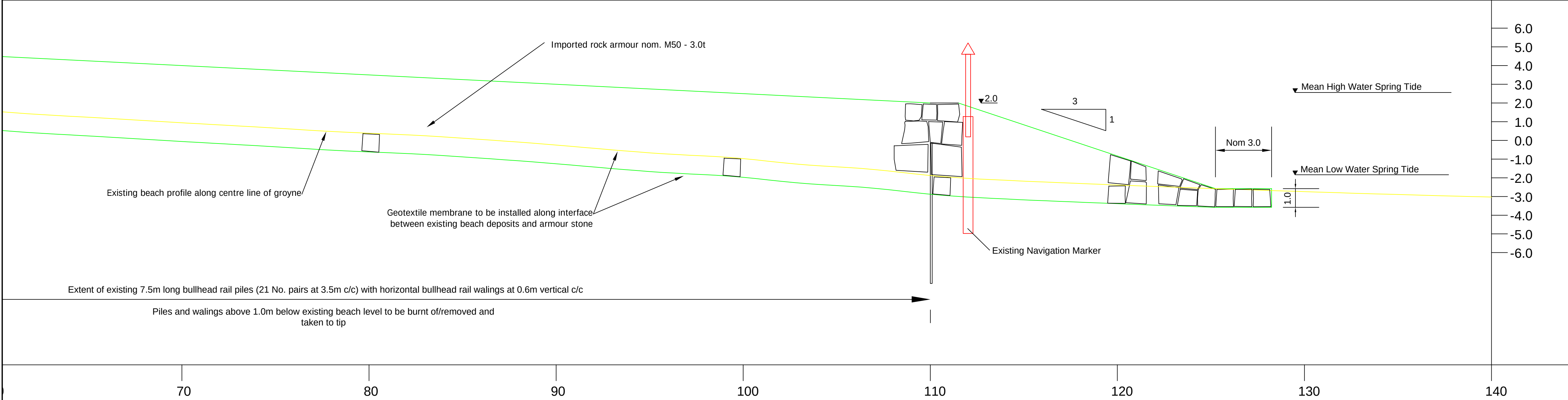
PWLLHELI HARBOUR CRIB GROYPE LONG SECTION 2/2 (1:125)
