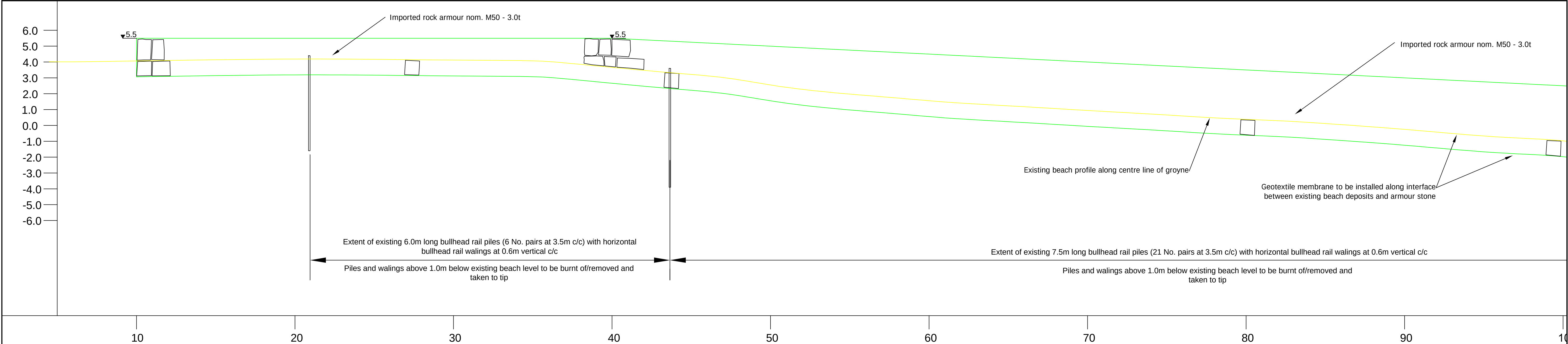
PWLLHELI HARBOUR CRIB GROYPE LONG SECTION 1/2 (1:125)
