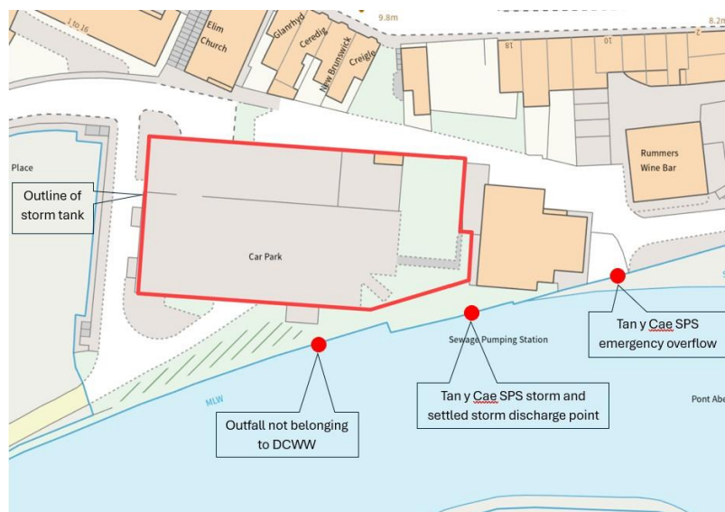
Figure 2: Revised figure of storm tank and outfalls at/near Tan y Cae SPS
