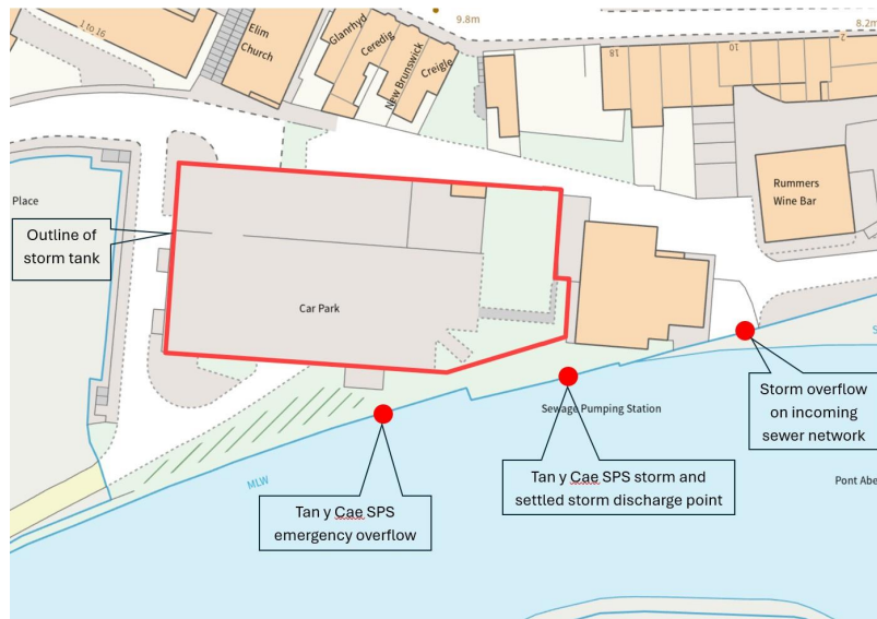
Figure 1: Storm tank and outfalls at/near Tan y Cae SPS supplied in CAR_NRW0049826
