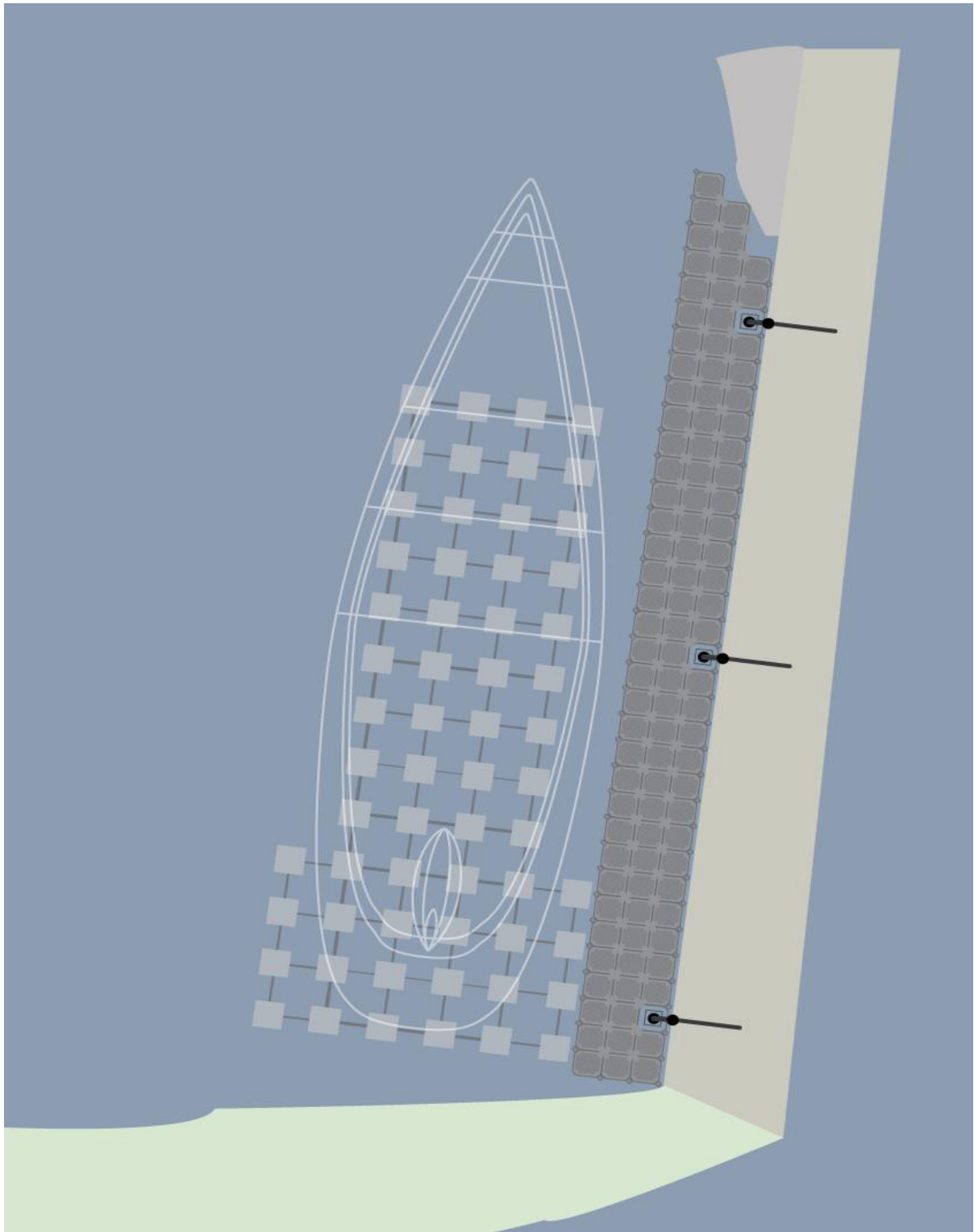
Plan showing location of piles, pontoon and cradle with respect to the boat and breakwater.
