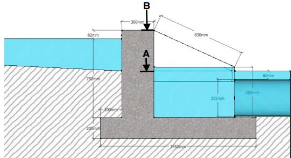
Point B: Proposed Height at Top of Weir Crest 325.789m AOD NGR (SN 86612 26167)
