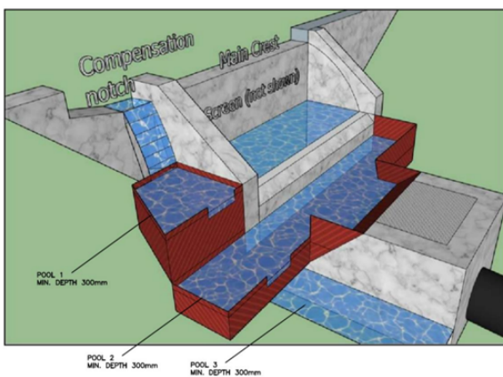
PICTORIAL VIEW EXTENT OF STEEL TRAY SHOWN IN DARK RED.
