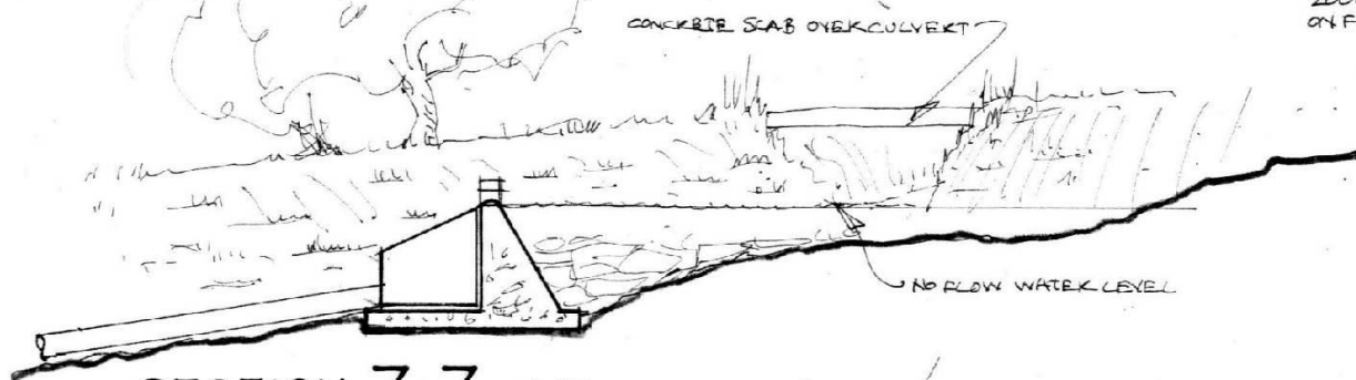
SECTION Z-Z 1:50
