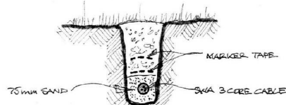
Type E - Cable in trench. 75mm Sand bed and surround. Two layers of marker tape above. Minimum 450mm cover (520mm in roads), this may be increased to 1000mm in areas of potential deep ploughing.
