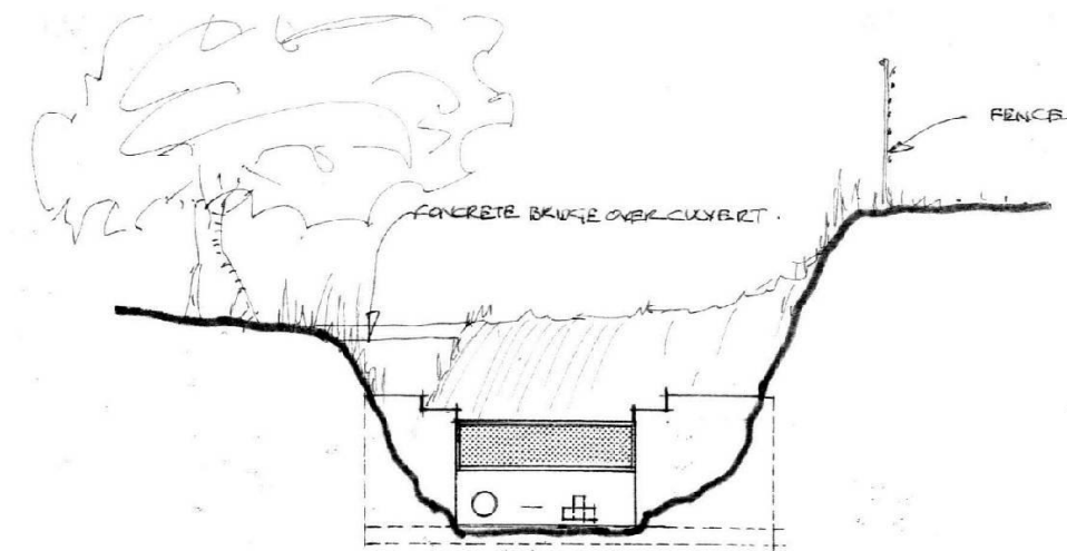
SECTION Y-Y 1:50
