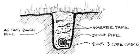
Type F - Cable in duct. Approved smooth bore duct with draw cord and long radius bends. Two layers of marker tape above. Minimum 450mm cover (520mm in roads), this may be increased to 1000mm in areas of potential deep ploughing.
