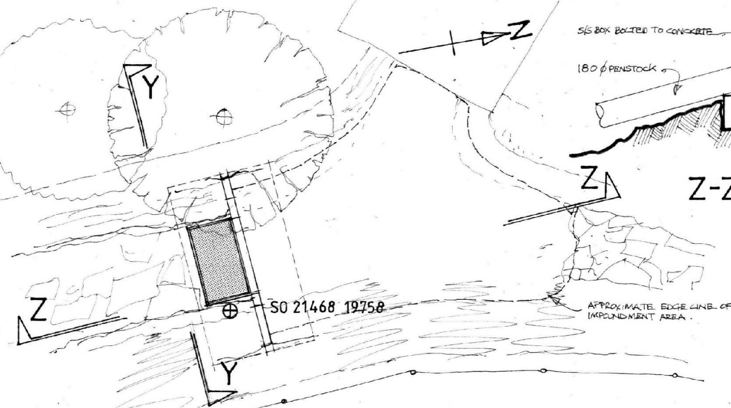
PLAN at INTAKE 1:50
