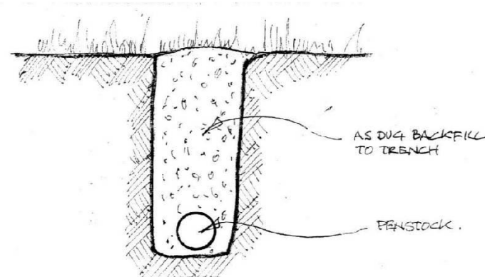
Type D - Pipe running along a long length of soft surface material running down a slope but without a cross slope and in a deeper trench. This like a traditional trench. Back fill to be selected excavated material with no sharp stones adjacent to the pipe. Cover to pipe to be a minimum of 450mm, this may be increased to 1000mm in areas of potential deep ploughing.
