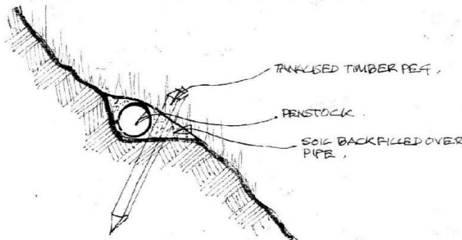
Type B - Pipe running along a long length of soft surface material but across a steep slope. Slope excavated to form 'shelf' upon which the pipe sits. Pipe held with tanalised timber pegs on the down slope side or with Stainless steel hoops. Excavated soil place back over the pipe to fill the gap on the upslope side of the pipe.
