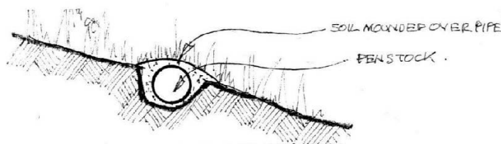
Type C - Pipe running along a long length of soft surface material running down a slope but without a cross slope and in a shallow trench. This will be similar to Type B but pipe 'shelf' will be a shallow trench with a depth of about 60% of the pipe diameter. Excavated soil is then piled up and over the pipe.
