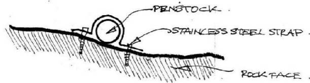
Type A - pipe running along a long length on a hard surface (in or out of stream). Pipe held in place with stainless steel straps drilled into hard surface (could be bed rock or just a large 'immovable' large boulder).
