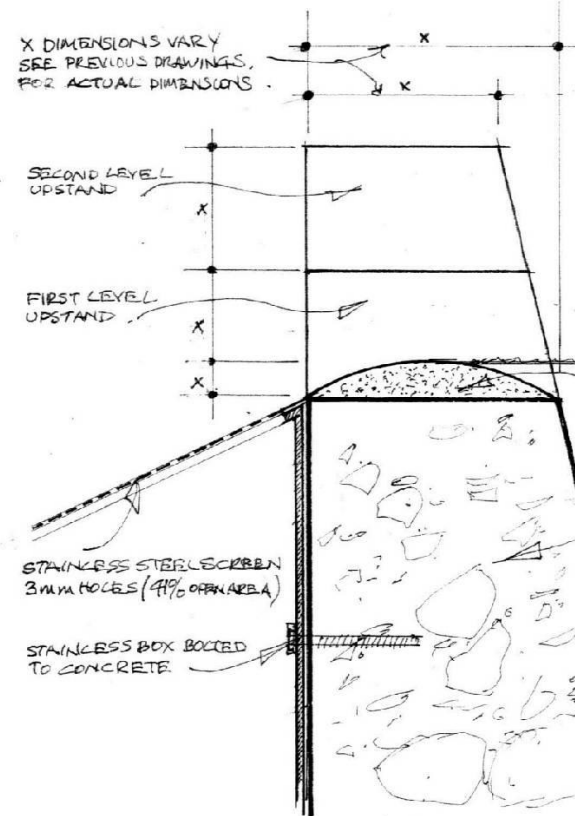
TYPICAL TOP OF WEIR INTAKE DETAIL 1:5
