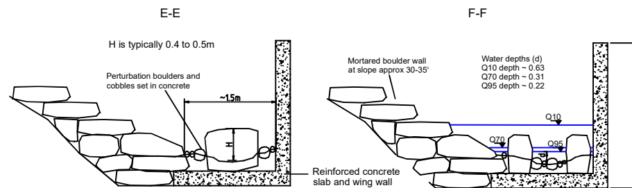
Typical Sections of Extended Bypass Channel to show Staggered Perturbation Boulders
