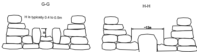
Typical Sections of Bypass Channel to show Staggered Perturbation Boulders
