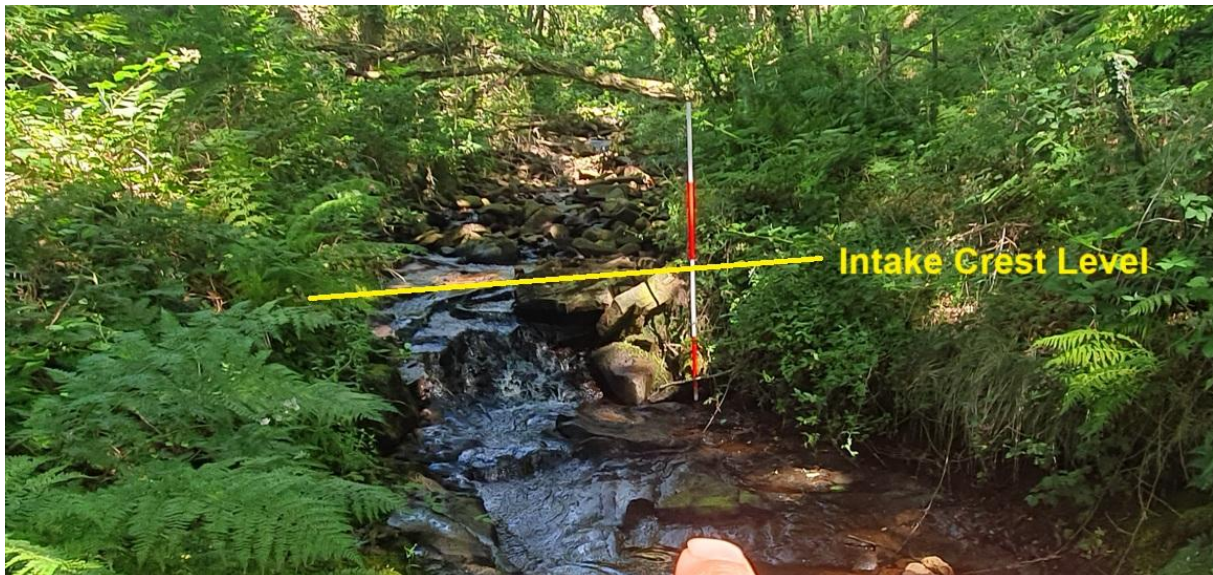
Intake Location with approximate crest level shown of proposed intake weir
