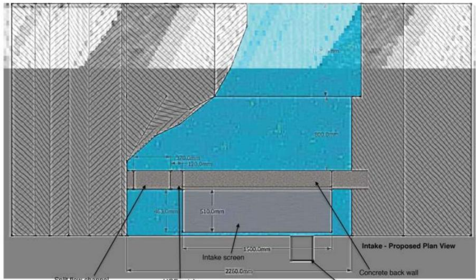
Split flow channel HOF notch Intake screen Intake - Proposed Plan View Concrete back wall 225mm external diameter high density polyethylene pipe
