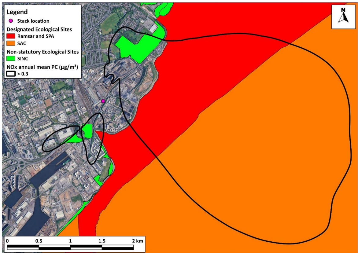
Figure 8-2: Contour Plot of Annual Mean NO x PC – Natural Gas
