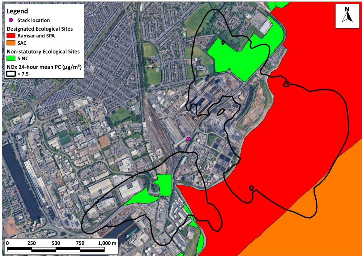
Figure 8-7: Contour Plot of 24-hour Mean NOx PC - Hydrogen
